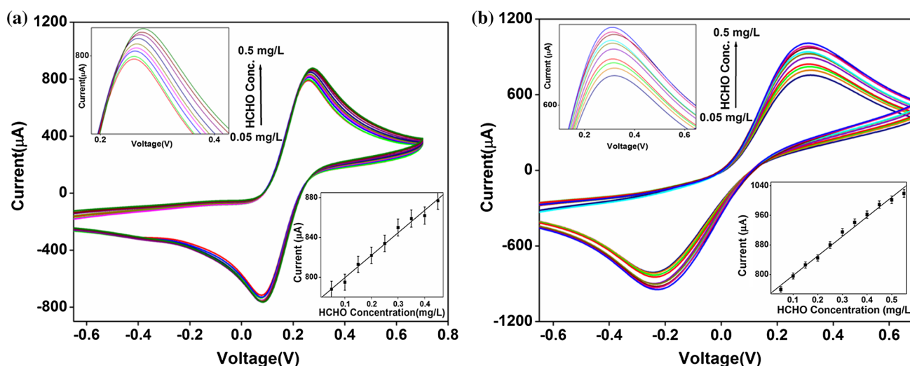
Fig. 4 Cyclic voltammetry studies of a BSA/FDH/CNT/ITO and b BSA/FDH/CNT-Fe 3 O 4 /ITO bioelectrodes as a function of formaldehyde concentrations from 0.05–0.50 mg/L, (inset image: a calibration curve of peak current value plotted against formaldehyde concentrations)
