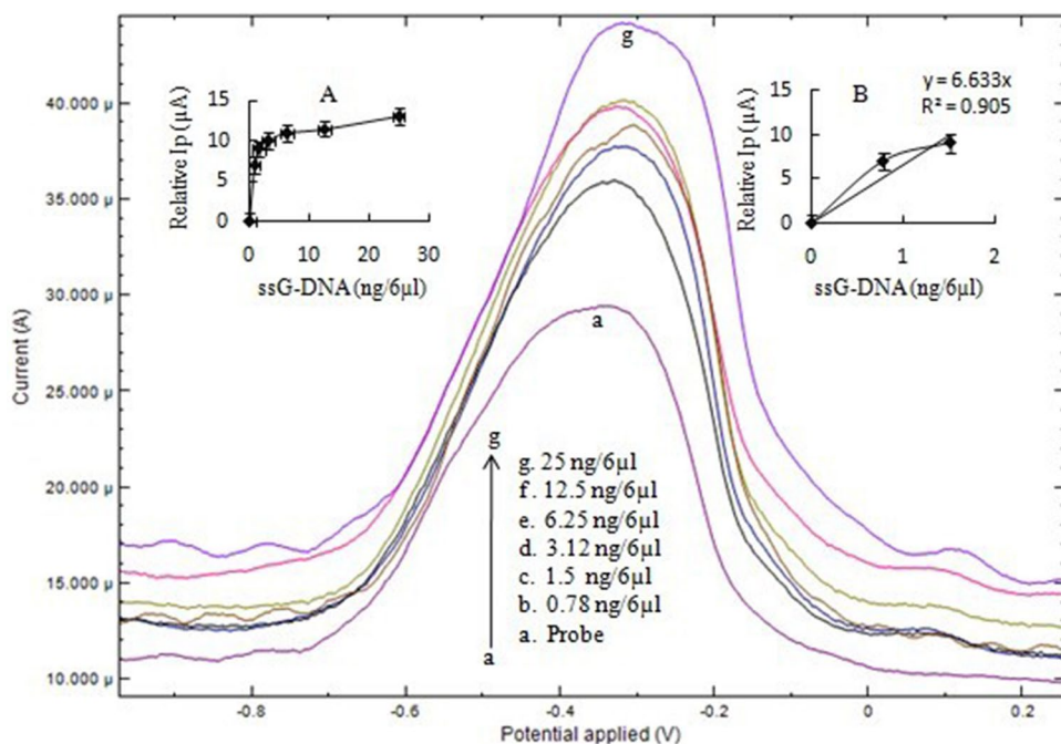
Fig. 3 DPV of (a) ssDNA-NH 2 /nano-Au/c-MWCNTs electrode and (b–g) hybridization with L. interrogans ssG-DNA using 1 mM MB in 50 mM PBS, pH 7. The inset a shows hyperbolic curve from 0 to 25 ng/6 \mu l with linear peak current ( I_p ) up to 1.5 ng/6 \mu l of ssG-DNA of L. interrogans . Inset b shows the linear plot from 0 to 1.5 ng/6 \mu l ssG-DNA for calculation of sensitivity and LOD
