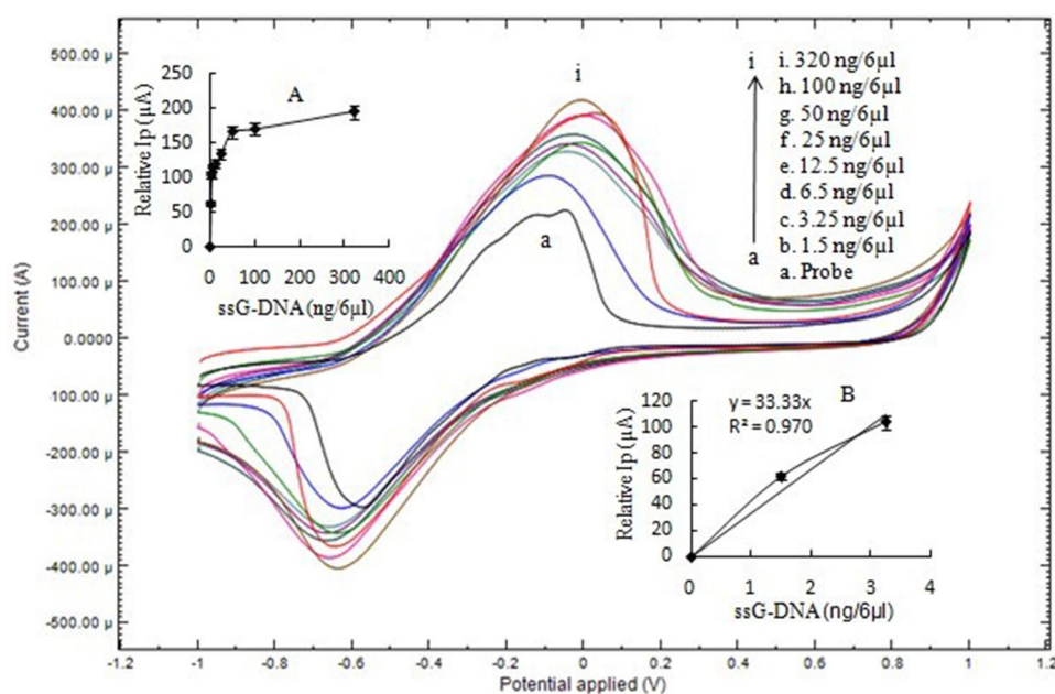
Fig. 2 CV of (a) ssDNA-NH 2 /nano-Au/c-MWCNTs electrode and (b–i) hybridization with of L. interrogans ssG-DNA at 50 mV/s using 1 mM MB in 50 mM PBS, pH 7. The inset a shows hyperbolic curve from 0 to 320 ng/6 \mu l with linear peak current ( I_p ) up to 3.25 ng/6 \mu l of ssG-DNA of L. interrogans . Inset b shows the linear plot from 0 to 3.25 ng/6 \mu l ssG-DNA for the calculation of sensitivity and LOD
