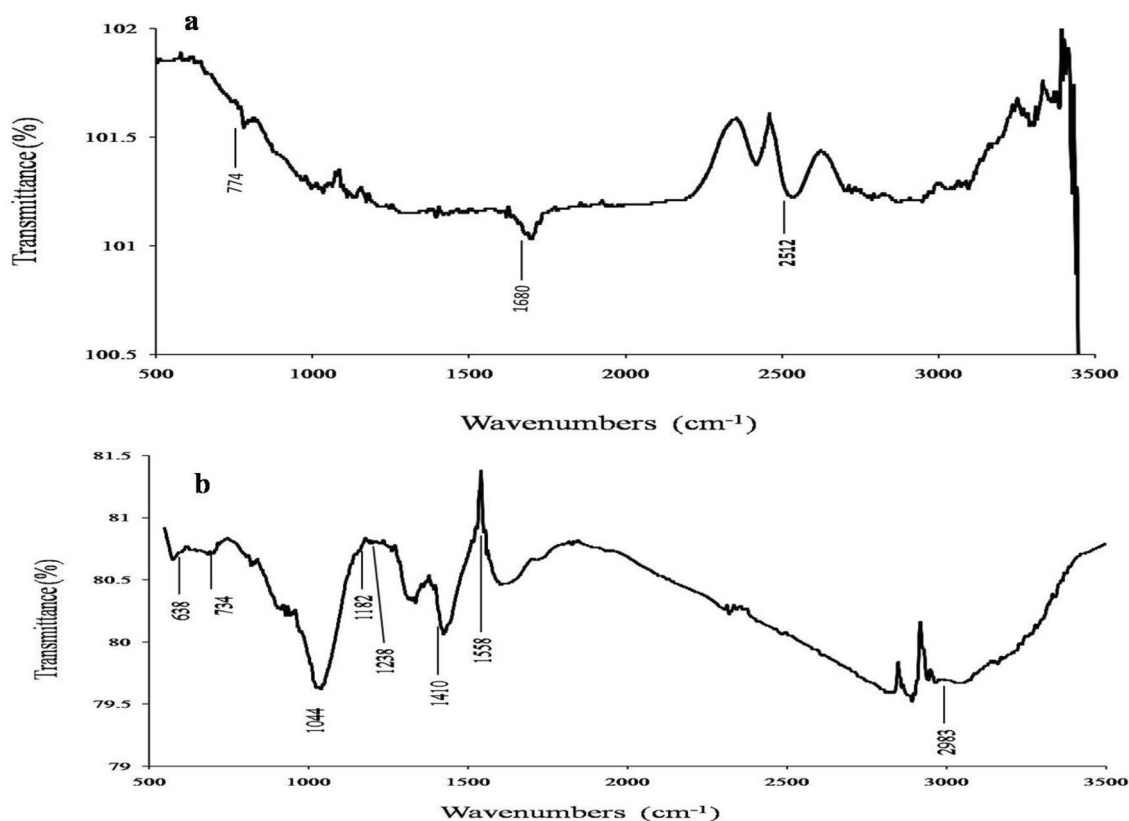
Fig. 5 FTIR spectra of a AuNPs-CNF and b AuNPs-CNF-ssDNA at frequency range of 500–3500 \text{cm}^{-1} ensures the immobilization of ssDNA probe onto the surface of AuNPs-CNF electrode
