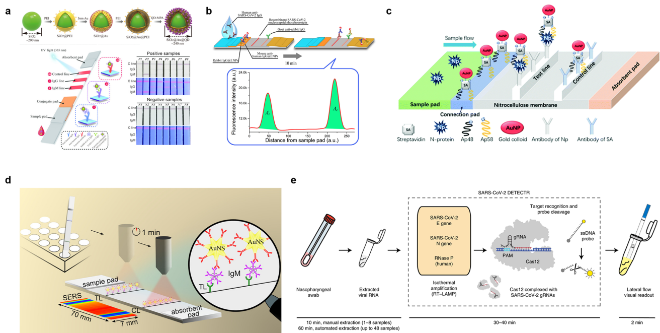
Fig. 6 a Fabrication process of the dual-mode SiO 2 @Au@QD and schematic of dual-mode LFA for detecting anti-SARS-CoV-2 IgM and IgG antibodies, reproduced with permission from [99], copyright 2020 ACS. b Lanthanide-doped nanoparticles-based LFA for detecting anti-SARS-CoV-2 IgG, reproduced with permission from [103], copyright 2020 ACS. c DNA aptamers-based LFA for detecting SARS-CoV-2 N antigen, reproduced with permission from [111],
