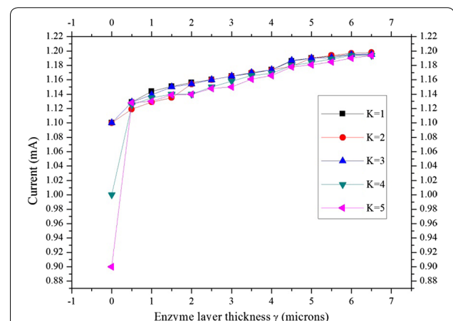
Fig. 3 Simulated currents as a function of the enzyme layer thickness for different reaction rate constant of D (represented as k in all the figures below) values measures up to 1, 2, 3, 4 and 5 s -1 from base to top
