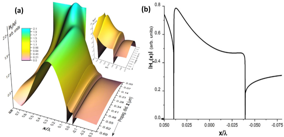
Fig. 3 a 3D plot for the propagated field and the inset shows the modal field in the metal film. b The magnitude of the magnetic field inside and around the metal film at the plane z=0.35 micron, where the magnitude of the plasmonic mode reaches its maximum value
