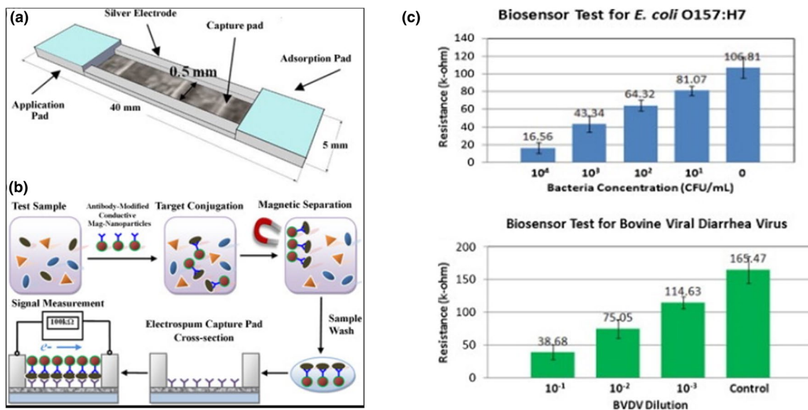
Fig. 5 A Diagram of the biosensor structure and membrane assembly made up of electrospun cellulose nitrate capture pads and cellulose application and absorption pads. B The lateral flow immunosensor's detection strategy based on an electrospun membrane with an
