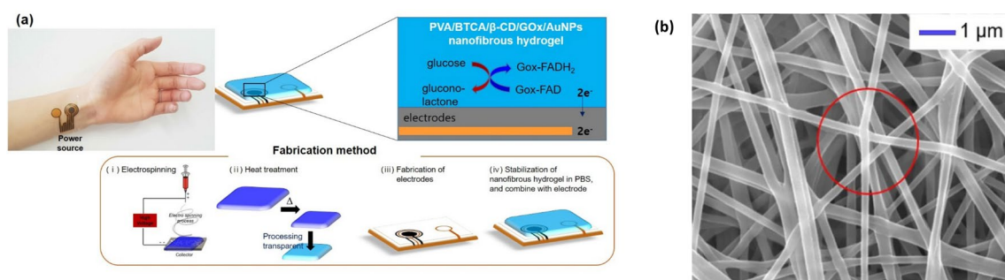
Fig. 6 a A non-invasive continuous monitoring biosensor fabrication method using electrospinning to applying an electrode for glucose sensing in sweat, b SEM characterization of nanocomposite PVA/BTCA/β-CD/GOx/AuNPs hydrogel nanofibers (poly(vinyl alcohol)
