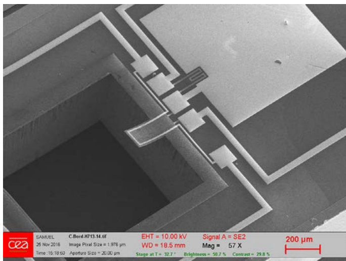
Fig. 5 Photograph of a microcantilever device fabricated by CEA, France. Microcantilever sensors operate by detecting changes in resonance response or deflection caused by mass loading, surface stress variation, or changes in damping conditions. Four resonance response parameters (resonance frequency, amplitude, Q-factor, and deflection) can be detected simultaneously. Surface stress produced as molecules adsorb on a cantilever can be observed as changes in deflections. Photograph—courtesy of Dr. Emmanuel Scorsonne, CEA, France.
