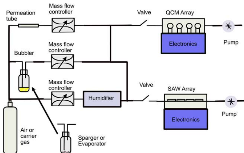
Fig. 11 Gas Rig for testing OBP sensors using either QCM or SAW platforms. Analyte generation may be through bubblers, permeation tubes, spargers, headspace stripping devices or others. The generated vapor is diluted with clean humidified air via mass flow controllers to produce desired concentration ranges of vapors to be applied to the sensors. A small pump aspirates vapor across the sensor arrays.
