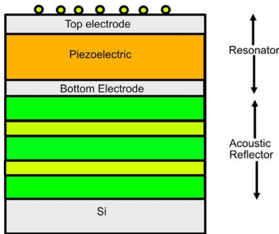
Fig. 4 The structure of a film bulk acoustic resonator (FBAR) is shown. Piezoelectric films fabricated using MEMS technology are thinner, can reach higher frequencies and offers the advantage of monolithic integration with advanced CMOS technology for peripheral readout and signal processing circuitry. FBARs are fabricated from a thin central piezo-electric layer with metal electrodes micropatterned on both sides. The FBAR's Q-factor can be increased by placing it on top of an acoustic mirror. The acoustic mirror is formed using alternating oxide and metallic layers. Acoustic isolation from the substrate is achieved when a Bragg reflector, comprised of layer pairs with contrasting acoustic impedance is placed underneath the FBAR. The exposed electrode at the top of the FBAR can be functionalized to immobilize proteins or other materials to create biosensors. Adapted from Voiculescu, I., & Nordin, A. N. (2012). Acoustic wave based MEMS devices for biosensing applications . Biosensors and Bioelectronics , 33(1), 1–9. https://doi.org/10.1016/j.bios.2011.12.041 .
