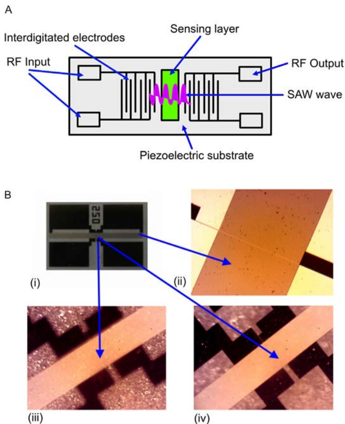
Fig. 3 (A) A schematic of a simple SAW resonator is shown. Two Interdigitated electrode structures (IDT) are deposited on a piezoelectric substrate. This makes up a SAW delay line. One IDT acts as the input or the transmitting IDT which converts radiofrequency (RF) electrical signals to acoustic energy that propagates on the surface of the piezoelectric substrate to the output (IDT) transducer which converts acoustic energy back to an electric signal creating a delay equivalent to the time taken by the surface acoustic wave to travel between the two IDTs. If an adsorbent material is placed between the two IDTs, then adsorption of molecules from the vapor phase on to the material will cause a change in the propagation delay of the surface acoustic wave. (B) (i) a SAW transducer manufactured by KIT (Karlsruhe Institute of Technology, Germany)—the band in the center running from left to right constitutes interdigitated electrodes shown in more detail in (ii) the gap between each electrode sets the resonant frequency of the structure. (iii) and (iv) show views of the SAW transducer modified by deposition of nanocrystalline diamond (CEA, France) which allows attachment of OBPs via NTA modified diamond surfaces. Panel (A) adapted from Voiculescu, I., & Nordin, A. N. (2012). Acoustic wave based MEMS devices for biosensing applications . Biosensors and Bioelectronics , 33(1), 1–9. https://doi.org/10.1016/j.bios.2011.12.041 .
