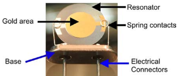
Fig. 2 An AT-cut 20MHz quartz crystal is shown. The resonator is supported by two spring contacts at the edges. These make electrical and mechanical contact with evaporated gold disks deposited on both sides of the QCM and are connected to the electrical contacts on the crystal base. The crystal sets the base frequency of an oscillator circuit that produces a train of electrical pulses at a frequency set by the resonant frequency of the crystal.
