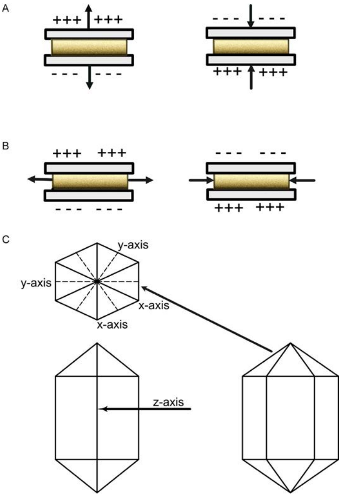
Fig. 1 The piezoelectric effect is illustrated; mechanical tension or compression on a piezoelectric material will induce a current depending type of stress and direction shown by the arrows shown in (A) and (B). When a stress is applied to a piezoelectric material, the dimensions of the material changes. Depending on the direction the stress is applied, the resulting change in dimensions can shift the centers of mass for the positive and negative ions; this produces a dipole throughout the material. The dipoles inside the material cancel each other out, but on the surface of the material the dipoles are not canceled out, producing a polarity between the faces of the material. (C) A quartz crystal has a hexagonal prism structure shown on the right. As shown on the left, the z-axis runs along the length of the crystal and is called the optical axis. The x-axis or the electric axis is parallel to a line bisecting the angles between adjacent prism faces. The y-axis, which is also known as the mechanical axis, shown in dotted lines, is at right angles to the face of prism and also to the x-axis.
