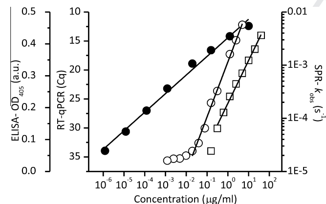
Fig.2. Comparison of the PVY detection and dose dependency using SPR (open squares), ELISA (open circles), and RT-qPCR (solid circles). In each case the virus concentration is plotted against the slope of the sensorgrams (SPR), the optical density at 405 nm after 1 h incubation with the substrate (ELISA), and the quantification cycle (C q ) for RT-qPCR. For each plot the data points that gave a linear regression with R_2 \geq 0.99 are depicted with a trend line.
