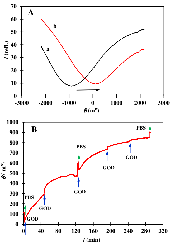
Fig.2. (A) The SPR angular scan curves for the GO before (a) and after equilibrium PANHS anchoring. (B) Real-time monitoring of the assembly of GOD on Au-coated SPR sensor surface modified by GO/PANHS. The down arrow (↓) indicates the point in time when GOD solution (4 \text{mg ml}^{-1} ) was introduced into the measurement cell and the up arrow (↑) represents the point in time at which the measurement cell was rinsed with 0.1 M PBS buffer (pH 7.0).
