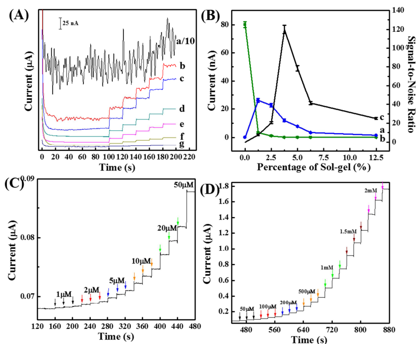
Fig. 3 A) Comparison of amperometric responses obtained from the GC/Au NFs/GS-IL-Au NRs (sol-gel a: 0%; b: 1.25%; c: 2.5%; d: 3.75%; e: 5%; f: 6.25%; g: 12.5%) electrodes towards 100 \mu\text{M} \text{H}_2\text{O}_2 , and B) The corresponding a) signal; b) noise; c) signal/noise of the electrodes in A. Attention: considering the noise in GC/Au NFs/GS-IL-Au NRs (sol-gel a: 0%) electrodes, we decrease their signal and noise into 10% here. C), D) Typical amperometric responses obtained by GC/Au NFs/GS-IL-Au NRs (sol-gel 3.75%) electrode with successive addition of specific concentrations of \text{H}_2\text{O}_2 from 1 \mu\text{M} to 2 mM.
