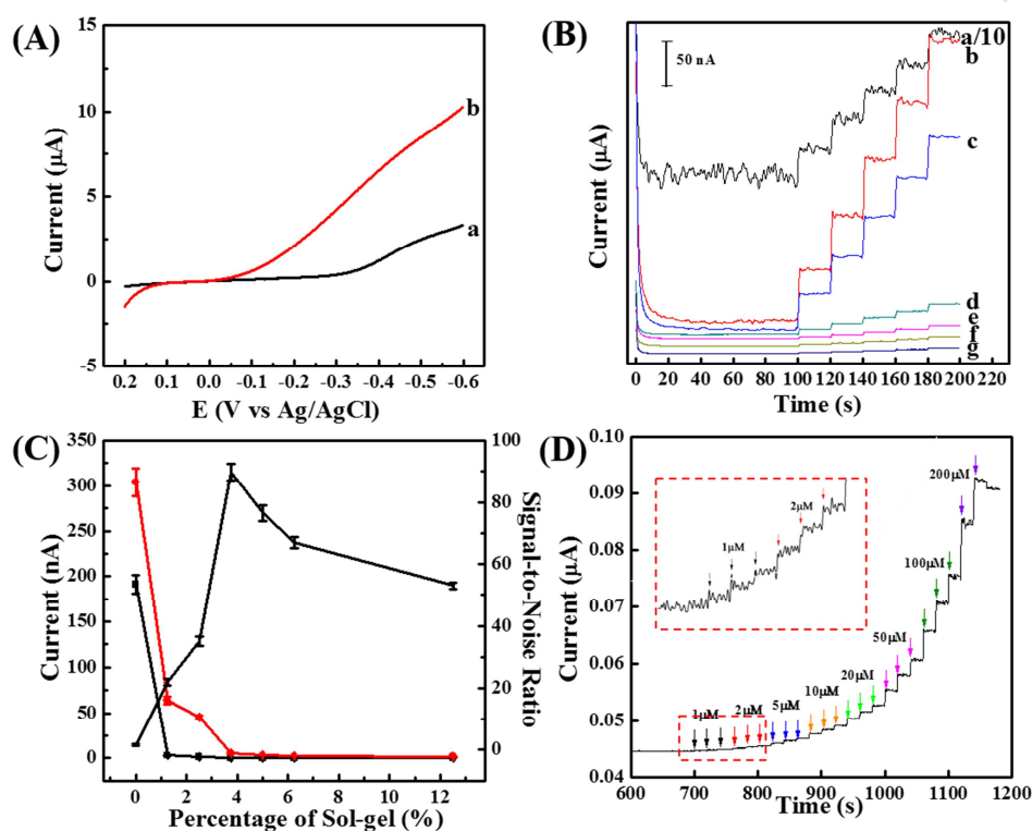
Fig. 4 A) LSV of GC/Au NFs/GS-IL-Au NRs (sol-gel 3.75%)/GOx biosensor toward 5 mM glucose in aCSF (a) without, (b) with 5 mM glucose. B) Comparison of amperometric responses obtained from the GC/Au NFs/GS-IL-Au NRs (sol-gel a: 0%; b: 1.25%; c: 2.5%; d: 3.75%; e: 5%; f: 6.25%; g: 12.5%)/GOx biosensors towards 100 \mu\text{M} glucose. and C) The corresponding a) signal; b) noise; c) signal/noise of with the increasing sol-gel in A. D) Amperometric responses obtained by GC/Au NFs/GS-IL-Au NRs (sol-gel 3.75%)/GOx biosensor with successive addition of specific concentrations of glucose from 1 \mu\text{M} to 200 \mu\text{M} .
