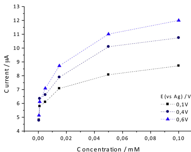
Fig. 1. Calibration curves obtained at different potential values using sensor # 9.
