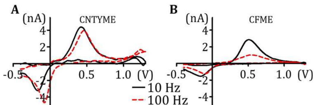
Figure 1. Comparison of the effect of FSCV scan repetition rate at (A) a carbon nanotube yarn disk microelectrode (CNTYME) and (B) a carbon fiber disk microelectrode (CFME). 1 \mu M dopamine is detected using a scan rate of 400 V/s. The repetition rate is either 10 Hz (solid black traces) or 100 Hz (dashed red traces). Carbon nanotube yarn electrodes are not dependent on scan repetition frequency. Adapted with permission from reference [47].
