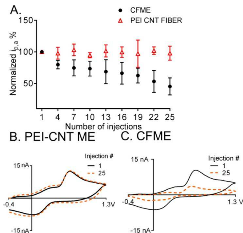
Figure 3. Serotonin fouling at a PEI-CNT fiber microelectrode. (A) Repeated injections of serotonin ( 1 \mu\text{M} ) every 15 s for 25 injections lead to no decrease in current for serotonin at PEI-CNT fiber electrodes (red) as opposed to the 50% decrease for carbon-fiber microelectrodes (CFMEs) (black). (B) Example cyclic voltammograms of 1 \mu\text{M} serotonin for a PEI-CNT fiber microelectrode for the 1st (solid black) and 25th injection (dashed red), approximately 6.25 min apart. The CVs are similar. (C) Example cyclic voltammograms of 1 \mu\text{M} serotonin at CFMEs for the 1st and 25th injection, indicating serotonin fouling does occur at the surface of the CFME. Adapted with permission from reference [68].
