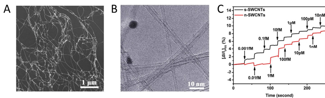
Figure 2. FET-based sensor for detection of dopamine. (A) SEM and (B) TEM images of the semiconducting SWCNTs (s-SWCNTs). (C) Typical real time current ( \Delta I/I_0 ) changes with dopamine concentration in a PBS solution for FET sensor with s-SWCNT and normal SWCNTs (n-SWCNTs). Adapted with permission from reference [51].
