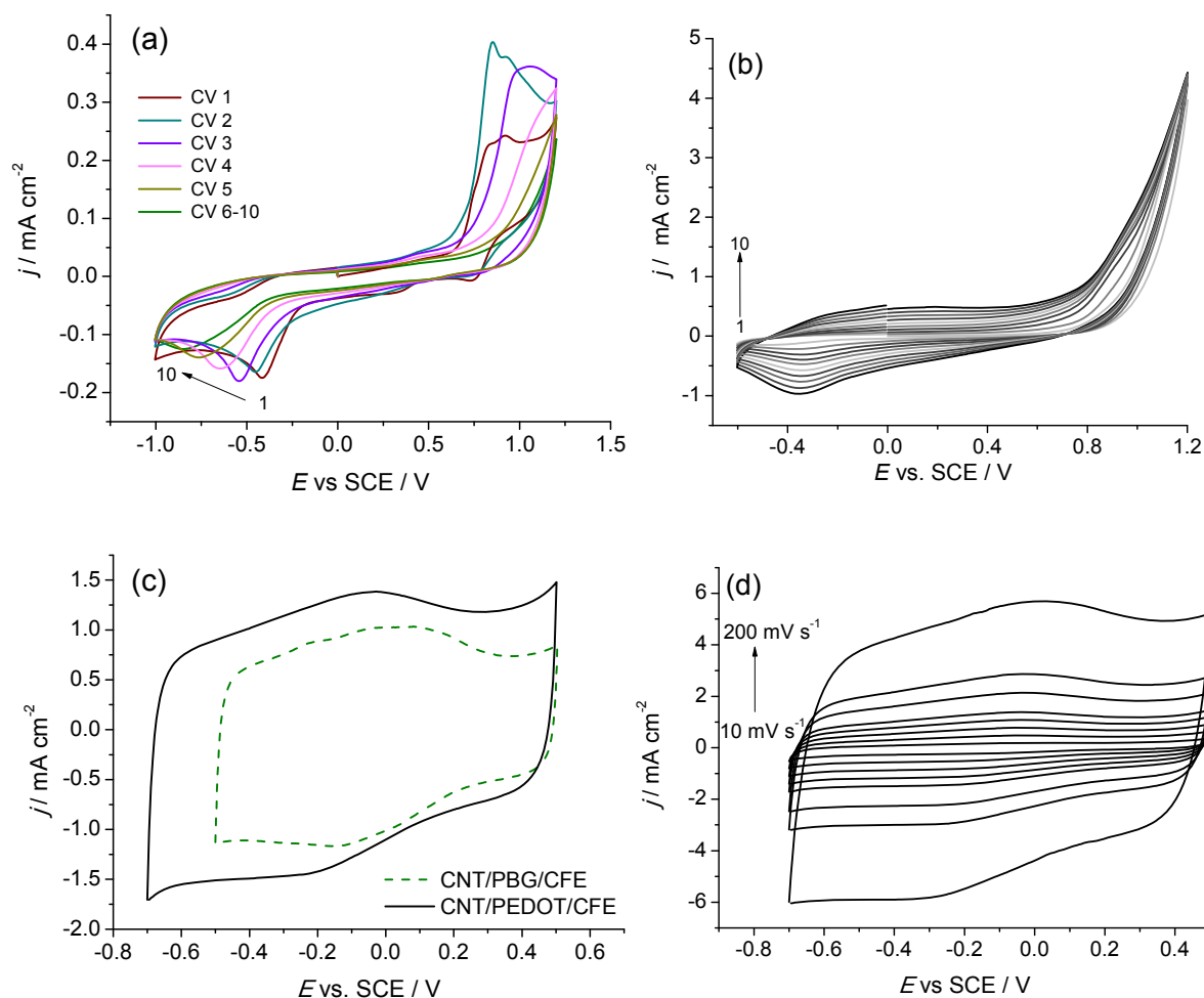
Fig. 1. Cyclic voltammograms obtained during polymerization of (a) BG (b) EDOT; CVs in 0.1 M KCl of (c) CNT/PBG/CFE and CNT/PEDOT/CFE at 50 \text{mV s}^{-1} and (d) CNT/PEDOT/CFE at different scan rates.
