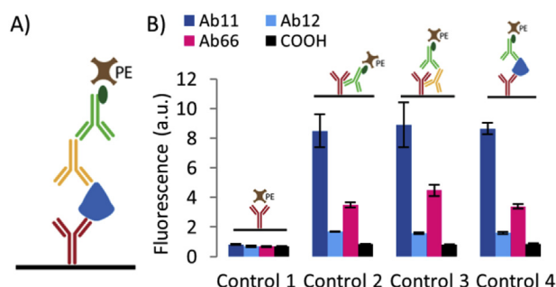
Fig. 1. A) Assay layout for the detection of nucleoprotein (blue) with capture antibody (red) immobilized on the \mu P surface. Signal was generated by sequentially introducing a secondary antibody (yellow), biotinylated detection antibody (green) and SA-PE (brown). B) Aspecific interaction between the capture antibodies Ab11 (dark blue), Ab12 (light blue) and Ab66 (pink) and other assay components. Error bars are standard deviations of three repetitions. (For interpretation of the references to colour in this figure legend, the reader is referred to the web version of this article.)
