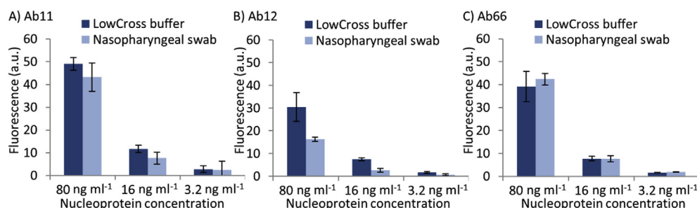
Fig. 4. Nucleoprotein detection in nasopharyngeal swabs (light blue bar) and LC buffer (dark blue bar) for A) Ab11, B) Ab12 and C) Ab66. Swabs of healthy people were diluted 10 fold in LC buffer and spiked with different concentrations of recombinant nucleoprotein (80, 16 and 3.2 ng mL -1 ). Incubation time for nucleoprotein was 15 min. Error bars are standard deviations of three repetitions. (For interpretation of the references to colour in this figure legend, the reader is referred to the web version of this article.)
