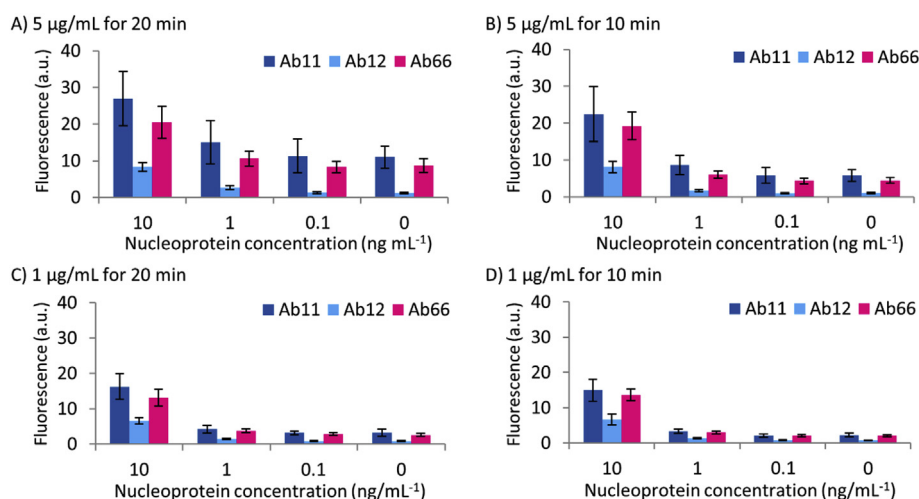
Fig. 2. Comparison of the different incubation conditions for the detection antibody A) 5 \mu\text{g mL}^{-1} for 20 min, B) 5 \mu\text{g mL}^{-1} for 10 min, C) 1 \mu\text{g mL}^{-1} for 20 min and D) 1 \mu\text{g mL}^{-1} for 10 min. Nucleoprotein (0.1, 1 and 10 \text{ng mL}^{-1} ) was incubated for 30 min. The results are shown for Ab11 (dark blue), Ab12 (light blue) and Ab66 (pink). Error bars are standard deviation of the average signal obtained for all \mu\text{Ps} per antibody population. (For interpretation of the references to colour in this figure legend, the reader is referred to the web version of this article.)
