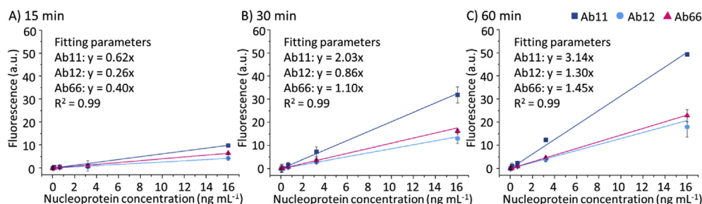
Fig. 3. Calibration curves of nucleoprotein detection in LC buffer for A) 15 min, B) 30 min and C) 60 min incubation time with the capture antibodies (Ab11 (dark blue), Ab12 (light blue) and Ab66 (pink)). Five-fold dilutions of the nucleoprotein were tested, starting from 80 \text{ng mL}^{-1} , of which the linear part (0.026 \text{ng mL}^{-1} to 16 \text{ng mL}^{-1} , i.e. five different concentrations) is shown here. The fluorescent signal was corrected for the background signal of the respective antibodies (i.e. 8.54 \pm 1.17 for Ab11, 1.92 \pm 0.12 for Ab12 and 0.75 \pm 0.95 for Ab66). Error bars are standard deviation of three repetitions. (For interpretation of the references to colour in this figure legend, the reader is referred to the web version of this article.)
