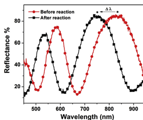
Fig. 2. Reflectance spectra of the etalon before and after reacting with AP-GAM solution. In this case, the AP-GAM solution was obtained after reaction with 0.1 \mu\text{g} mouse IgG (1.1 nM). The stars above the respective spectra indicate the position of the reflectance peaks before and after exposure of the etalon to excess AP-GAM.
