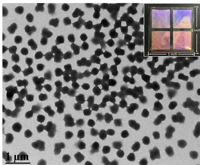
Fig. 1. TEM image of the microgels. Insert is a photo of a representative dry etalon used for performing the immunoassay.
