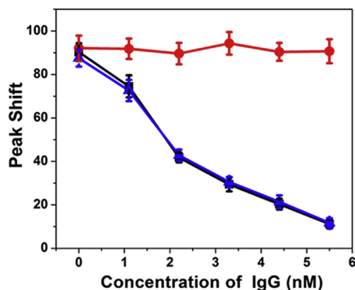
Fig. 3. Peak shift of the reflectance spectrum from the etalon as a function of IgG concentration (■ for mouse IgG, ● for rabbit IgG and ▲ for mouse IgG in the presence of rabbit IgG). Each data point is the average obtained from three individual experiments, and the error bars are the standard deviations of the measured values. We point out that the lines drawn through the data in the plot are meant to guide the eye, and are not model fits to the data.
