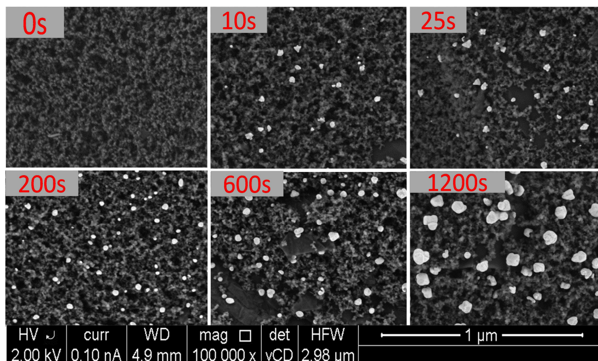
Figure 2. SEM images of the carbon working area of SPCEs after different gold electrodeposition times (from 0 to 1200 seconds). Precursor: 0.01% \text{HAuCl}_4 solution. Deposition potential: -0.4\text{ V} .
