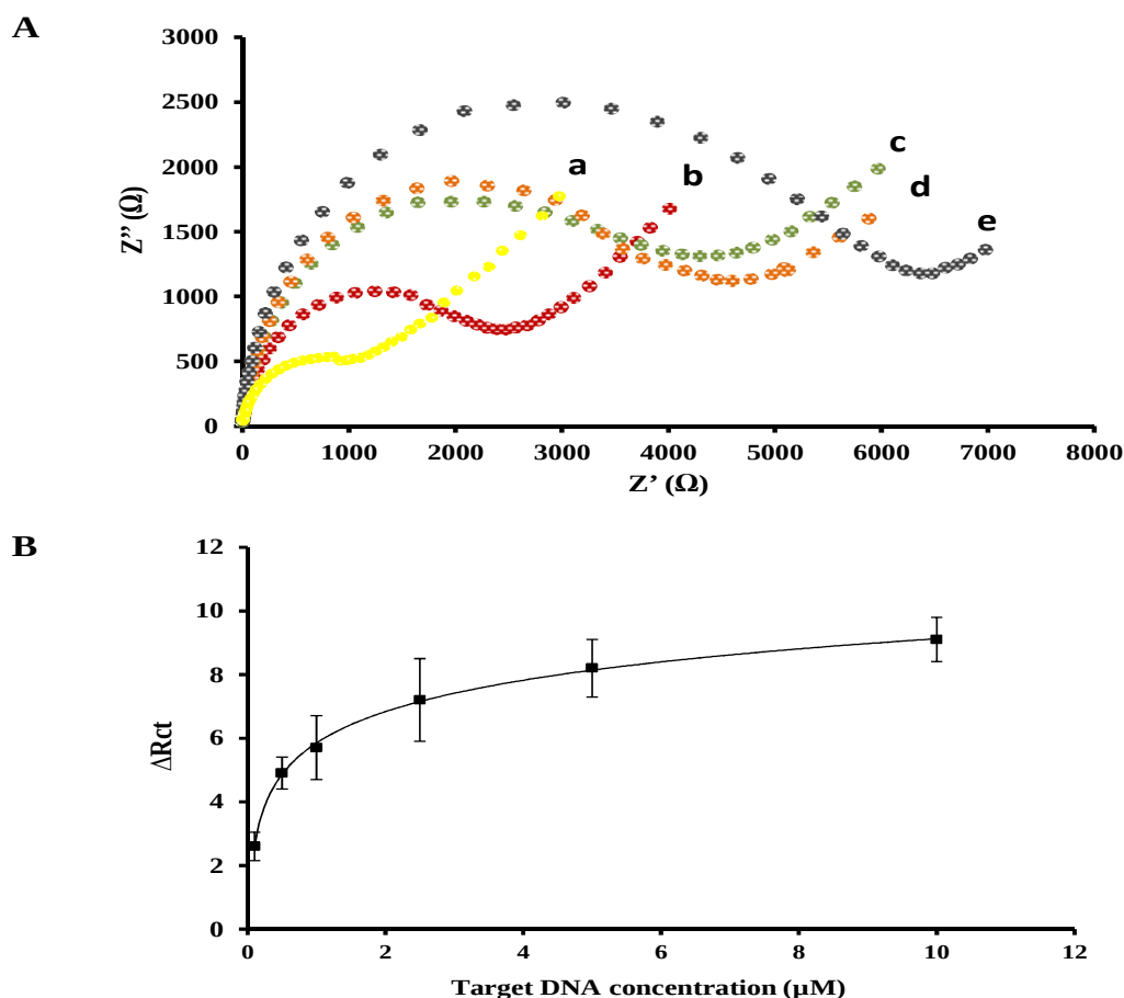
Figure 5. A) Nyquist plots recorded for control DNA a) and CTV-related ssDNA concentrations of 0.1 \mu\text{M} b) , 0.5 \mu\text{M} c) , 1 \mu\text{M} d) and 10 \mu\text{M} e) . Electrolyte: 0.5 mM \text{K}_3[\text{Fe}(\text{CN})_6]/\text{K}_4[\text{Fe}(\text{CN})_6] containing 0.1 M KCl; Potential: 0.2 V; Amplitude: 5 mV; Frequency range: 10 KHz to 0.5 Hz. B) Calibration curve obtained by plotting the normalized R_{ct} values vs the logarithm of different CTV-related DNA concentrations in the range of 0.1 to 10 \mu\text{M} . Other experimental conditions as described in the text.
