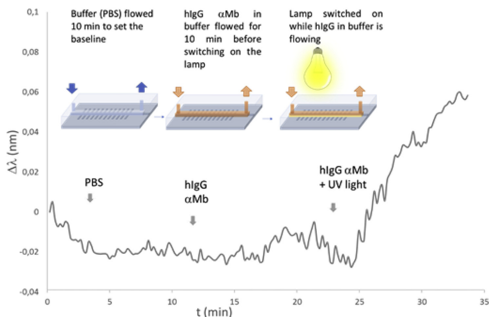
Fig. 7. Photochemical binding of hlgG antiMyoglobin ( \alpha Mb) antibody fragments detected in a label-free format by means of PBG optical sensor. Signal ( \Delta\lambda ) remains constant as long as buffer or hlgG flows over the alkene-derivatized optical chip, but a clear signal increase is registered when irradiating at 254 nm, what indicated the attachment of the thiolated probes to the surface.
