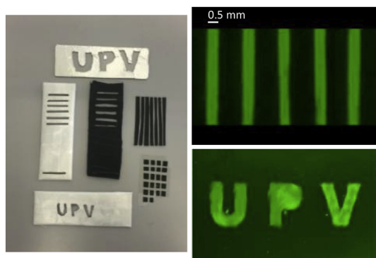
Fig. 2. Image of some of the handmade masks used to demonstrate the photomasking capability of the developed approaches (left) and fluorescence images obtained when irradiating through the photomask an alkynylated (top right) and epoxylated (bottom right) functionalized surfaces with a solution of labeled thiolated oligonucleotide spread out over the surface.
