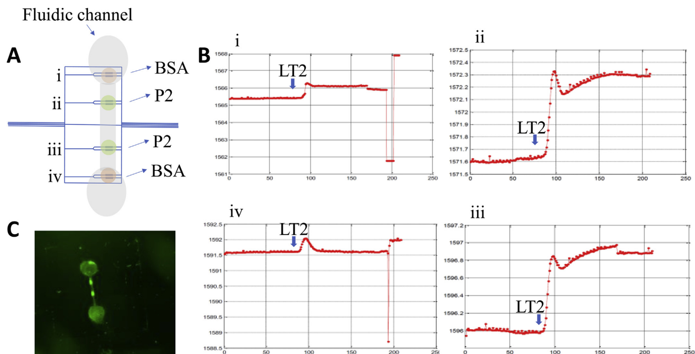
Fig. 6. A) Scheme of the nanophotonic sensing chip consisting of 4 pairs of PBG sensing structures. Outer pairs were biofunctionalized with BSA and inner pairs with thiolated probe 2 (P2); B) Spectral shift of the edge of the PBG observed for one sensor of each pair when labeled target 2 (LT2) was flowed over the sensors at 0.5 \mu M in SSC 1 \times ; C) Fluorescence image of the chip with the fluidic channel after performing the biosensing experiment.
