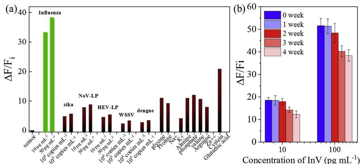
Fig. 5. (a) Selectivity test of the CdZnSeS/ZnSeS QD-peptide-AuNP biosensor with anti-influenza antibody. Used influenza virus, NoV-LP and HEV-LP were 10\text{--}50\text{ pg mL}^{-1} ; Zika, WSSV and Dengue virus of 10^4\text{--}10^5\text{ copies mL}^{-1} . Other common interfering was tested with metal ions ( 0.1\text{ mg mL}^{-1} ) and amino acids ( 2\text{ mM mL}^{-1} ), (b) Stability of the CdZnSeS/ZnSeS QD-peptide-AuNP nanocomposites towards 10 and 100\text{ pg mL}^{-1} influenza virus over 1-month period.
