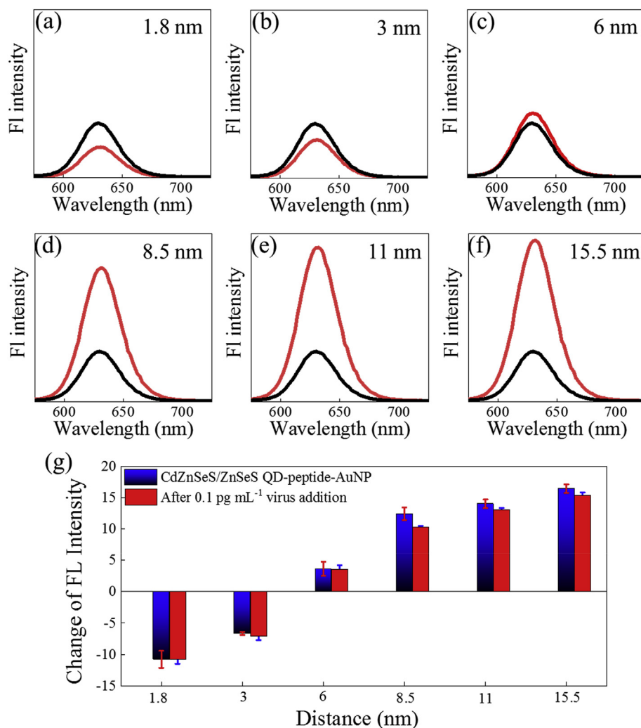
Fig. 3. Distance-dependent fluorescence spectra where the peptide length was varied from (a) 1.8, (b) 3, (c) 6, (d) 8.5, (e) 11 and (f) 15.5 nm (the black and red lines represent the fluorescence of CdZnSeS/ZnSeS QD-peptide before and after conjugation with AuNPs, respectively) and comparison of the change of fluorescence intensities with respect to the (g) linked peptide chain length variation and after addition of 0.1 pg mL -1 Influenza virus. (For interpretation of the references to color in this figure legend, the reader is referred to the Web version of this article.)
