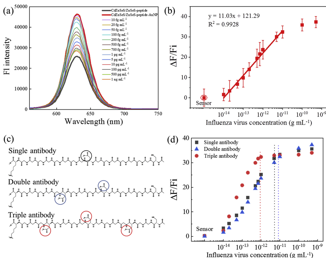
Fig. 4. (a) Fluorescence emission spectra for the detection of influenza viruses in the concentration range of 10^{-14} – 10^{-9} \text{ g mL}^{-1} using the LSPR-based CdZnSeS/ZnSeS QD-peptide-AuNP sensing probe. (b) Corresponding calibration curve for detection of the influenza virus with respect to the change of fluorescence intensity. Error bars denote standard deviation of 3 replicate measurements. (c) Used peptides with different number of carboxyl group. (d) Effect of one, double and triple antibody-conjugated sensing probe on sensing performance.
