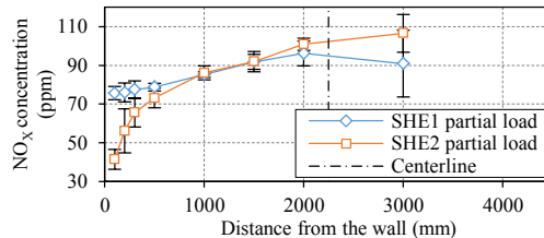
Fig. 5. NO x concentration profile – side walls of the furnace
