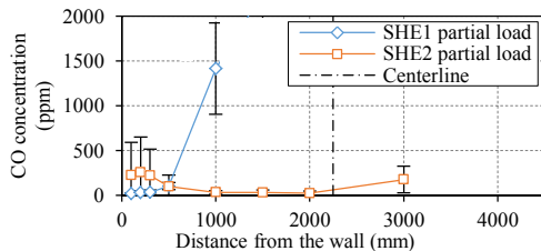
Fig. 4. CO concentration profile – side walls of the furnace
