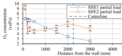
Fig. 3. O 2 concentration profile – side walls of the furnace
