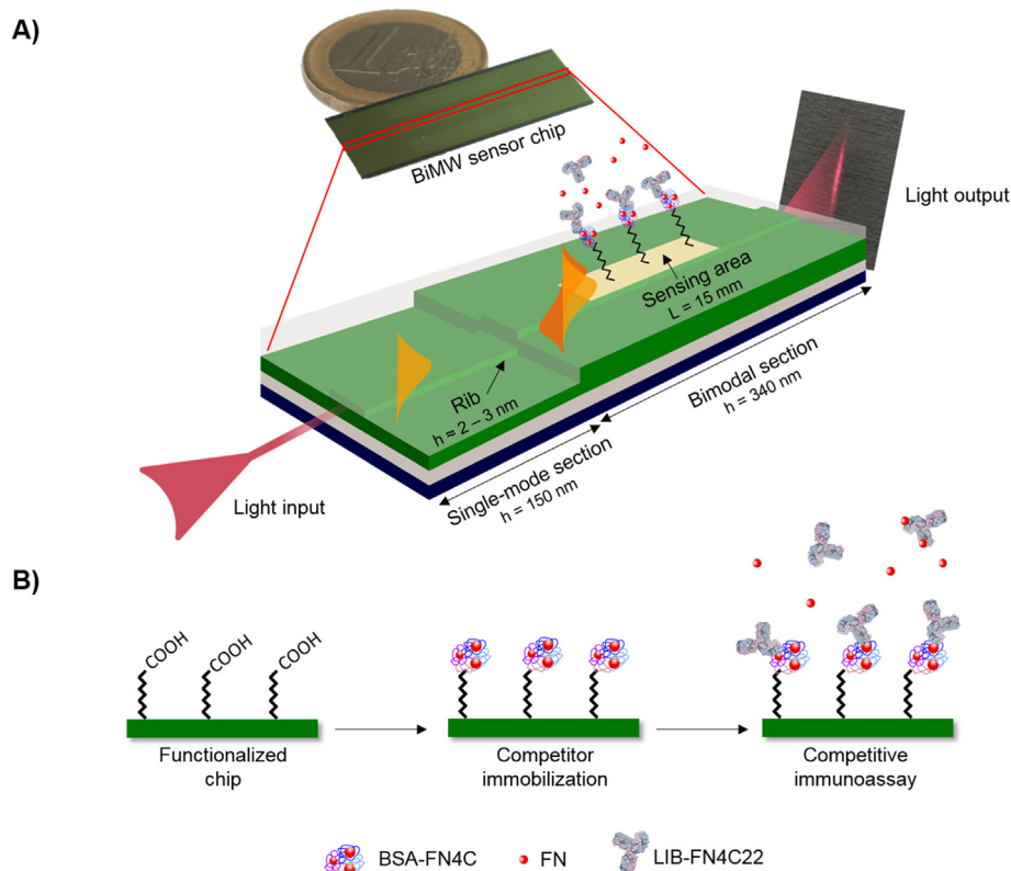
Fig. 2. (A) Photograph of a BiMW sensor chip. Zoom in one of the bimodal waveguides shows a schematic representation of the interferometer characteristics and the working principle. (B) Representation of the three main steps in the development of a competitive immunoassay for the detection of FN: functionalization of the sensor chip with silane-PEG-COOH; covalent immobilization of hapten-protein conjugate (BSA-FN4C competitor) and competition step with the sample containing a fixed concentration of antibody (LIB-FN4C22) and FN as target analyte.
