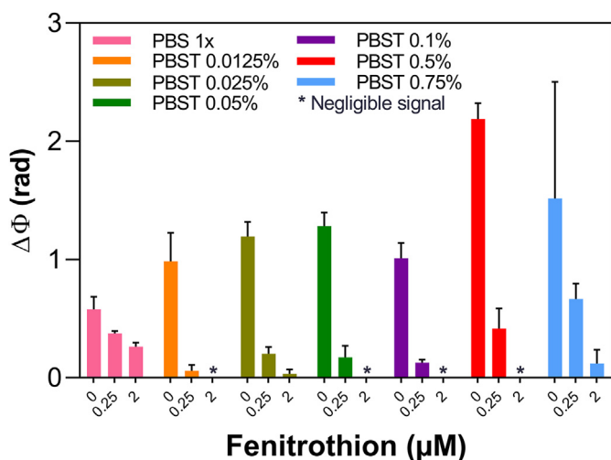
Fig. 3. Results obtained from the indirect competitive immunoassay for different FN concentrations (0, 0.25, and 2 \mu\text{M} ) pre-incubated with the antibody in different buffers: PBS and PBST with 0.0125–0.75% of Tween 20. [BSA-FN4C] = 20 \mu\text{g mL}^{-1} ; [LIB-FN4C22] = 1 \mu\text{g mL}^{-1} (Each column represents the mean \pm SD of duplicates).
