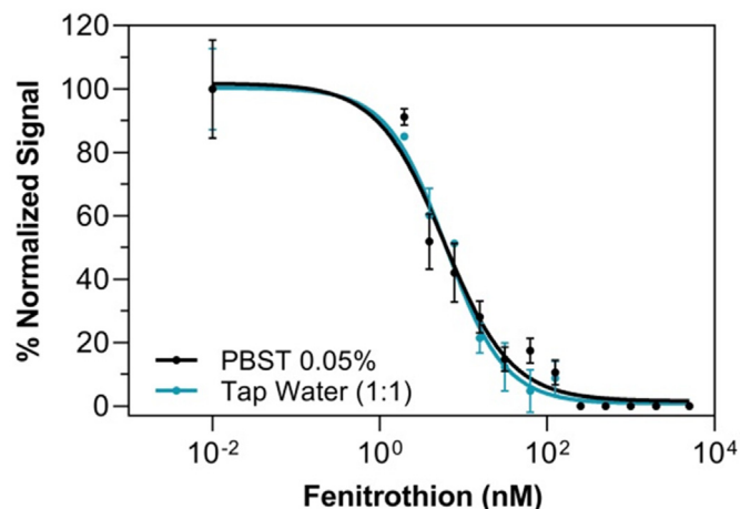
Fig. 5. Calibration curves for FN detection in PBST 0.05% (black) and tap water (1:1, blue). Each point represents the mean \pm SD of three replicates. (For interpretation of the references to colour in this figure legend, the reader is referred to the Web version of this article.)
