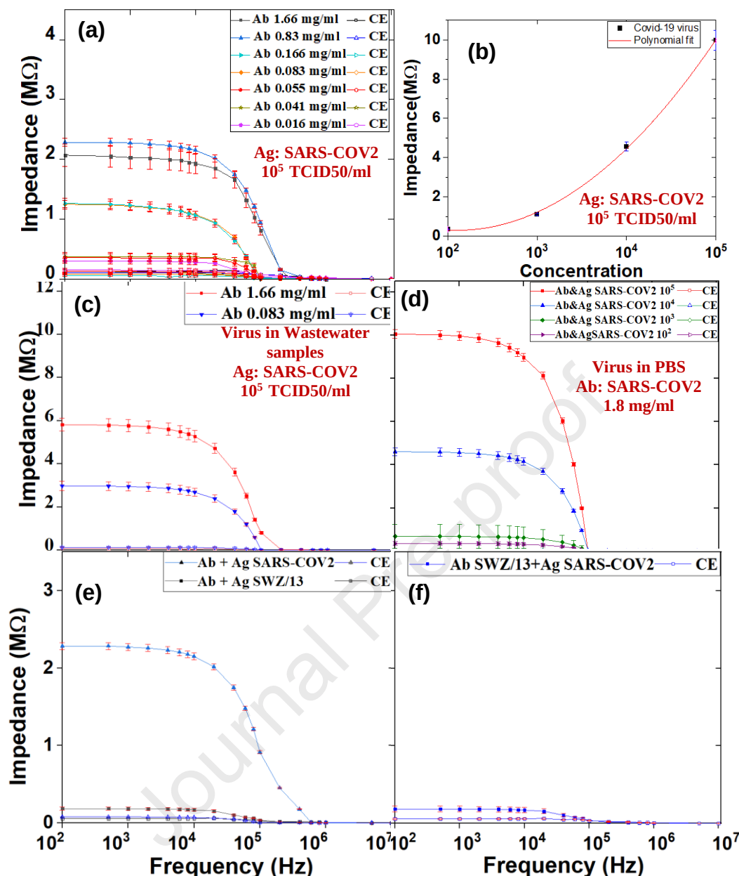
Figure 5. (a) The optimal antibody concentration against SARS-CoV-2 virus was determined using multiple antibody dilutions from 0.0166 mg/ml to 1.66 mg/ml mixed with a cross linker (Sulfo-LC-SPDP). Each antibody dilution was tested using a fixed virus concentration at 10 5 TCID 50 /ml in PBS and a fixed antibody coating time, i.e., 60 minutes. (b) The impedance change was plotted versus antibody concentration at 1 kHz. (c) The optimal antibody concentration against SARS-CoV-2 virus was determined using wastewater samples spiked with fixed concentration of SARS-CoV-2, i.e., 10 3 TCID 50 /ml. (d) Testing of SARS-CoV-2 in PBS at various titers. (e) The specificity was tested by immobilizing antibody (Ab) SWZ/13 against influenza virus (1.3 μg/ml) on the sensing electrode while SARS-CoV-2 samples with a fixed concentration of 10 5 TCID 50 /ml in PBS were used. The result was compared with detection of the SARS-CoV-2 antigen using SARS-CoV-2 antibody for the same antigen concentration. (f) The selectivity was measured using influenza virus samples with a concentration of 10 6 TCID 50 /ml with the sensing electrode coated with SARS-CoV-2 antibody (0.083 mg/ml).
