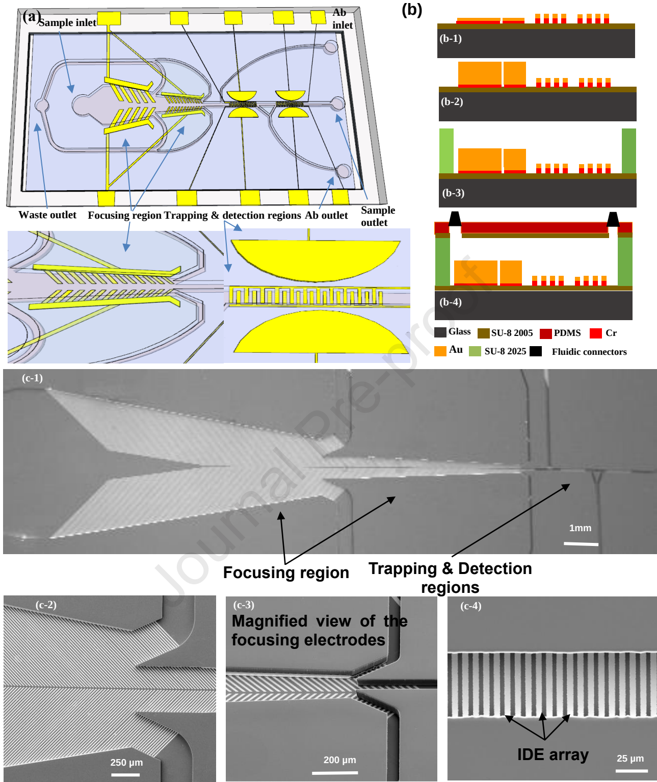
Figure 2: (a) Three-dimensional (3D) Schematics of the biosensor, presenting the focusing, trapping and detection regions, (b) A side view of biosensor showing the materials used in device fabrication, (c) Scanning electron microscope (SEMs) micrographs of the fabricated biosensor.
