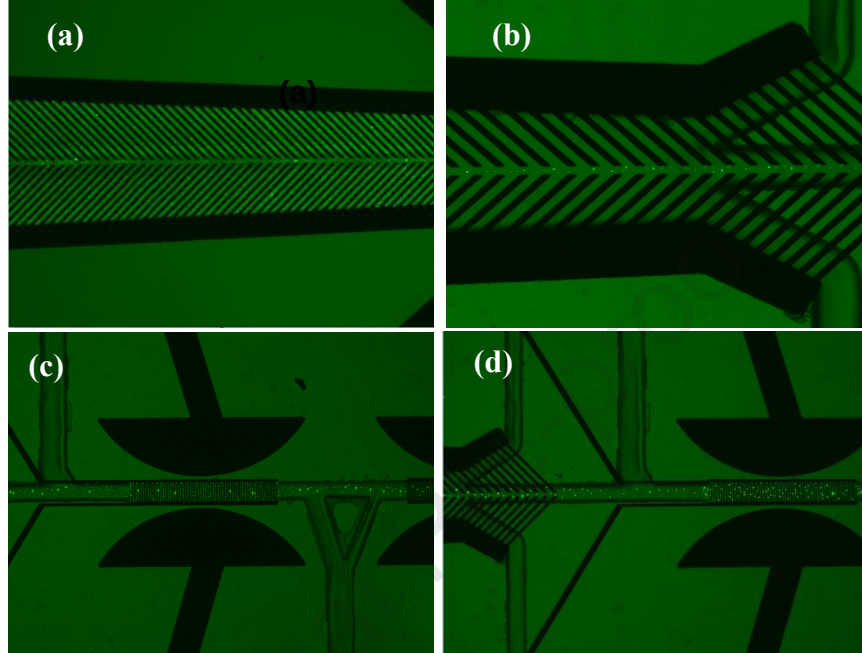
Figure. 4. (a) fluorescent images before focusing the nanobeads into the centerline of the focusing region, (b) fluorescent images after focusing the nanobeads into the centerline of the focusing region. (c) fluorescent images before trapping the nanobeads onto the surface of the detection electrode array. (d) fluorescent images after trapping the nanobeads onto the surface of the detection electrode array.
