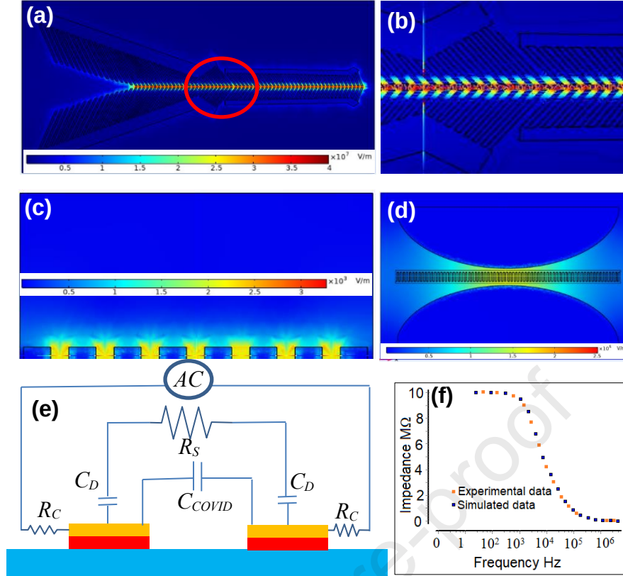
Figure 1. (a) An electric field (E-Field) modeling and simulation using COMSOL Multiphysics software of the three regions making the biosensor, i.e., (b) focusing, (c) detection regions and (d) tapping (e) An equivalent electrical circuit of the biosensor was also included in the simulation. (f) Finally, experimental and simulation results were obtained after the SARA- Covid-19 antibody-antigen binding occurred in the microchannel.
