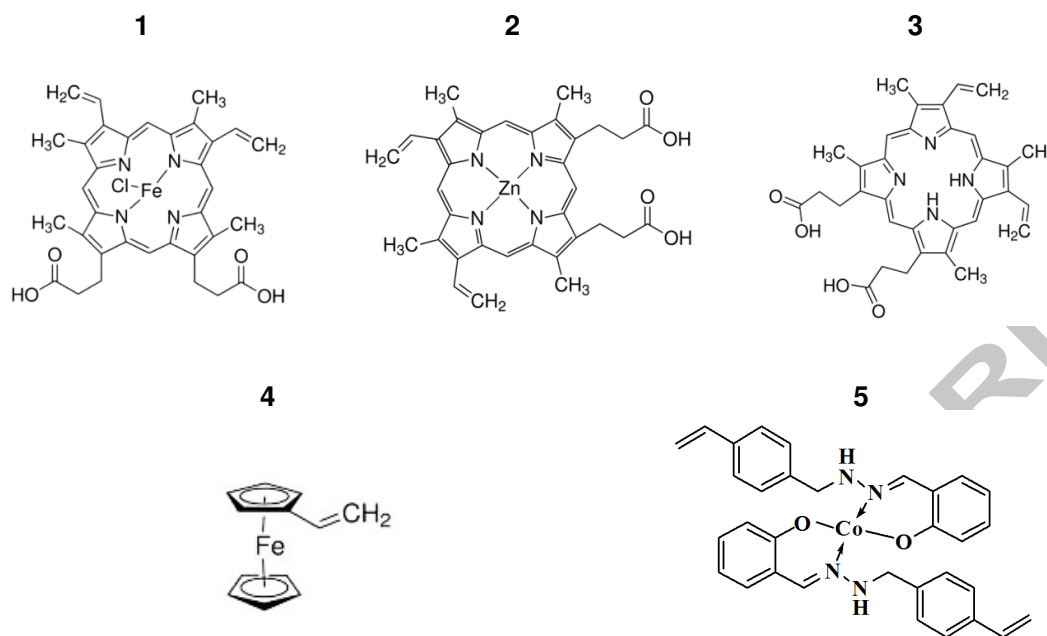
Figure 2 - Metal complex structures; 1 iron(III) chloroporphyrin IX (Hemin), 2 zinc(II) protoporphyrin IX (ZnPP), 3 protoporphyrin IX (PP), 4 vinylferrocene (VFc), 5 Co(II) complex (illustrating the (E)-2-((2 hydrazide-(4-vinylbenzyl)hydrazono)methyl)phenol ligand attachment via two nitrogen's).
