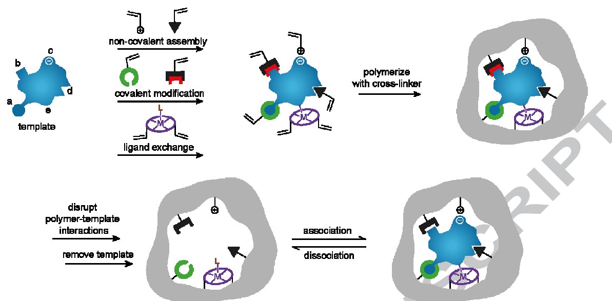
Figure 1 – Schematic representation of the imprinting process illustrating the reversible interactions between template and polymerizable functional monomers used in creating affinity. Depending on the synthetic strategy this may involve one or more of the following interactions: (a) reversible covalent bonds, (b) covalently attached polymerizable binding groups that are activated for non-covalent interaction by template cleavage (sacrificial spacer or semi-covalent strategy), (c) electrostatic interactions, (d) hydrophobic or van der Waals interactions, (e) co-ordination with a metal centre. Each, (a–e) respectively are formed with complementary functional groups or structural elements of the template. Subsequent polymerization in the presence of a cross-linker produces a porous matrix in which template sites are located; these can then be removed through disruption of polymer-template interactions (a–e), and extracted from the matrix. Template(s), or analogues thereof, may then be selectively rebound by the polymer in the sites/cavities vacated by template, or the imprints. Reproduced with permission from reference (2) .
