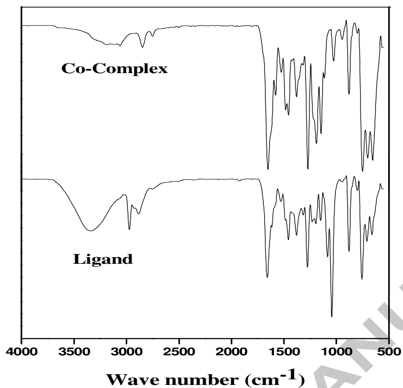
Figure 3 - FT-IR spectrum of the (E)-2-((2 hydrazide-(4-vinylbenzyl)hydrazono)methyl)phenol ligand and Co(II) complex.
