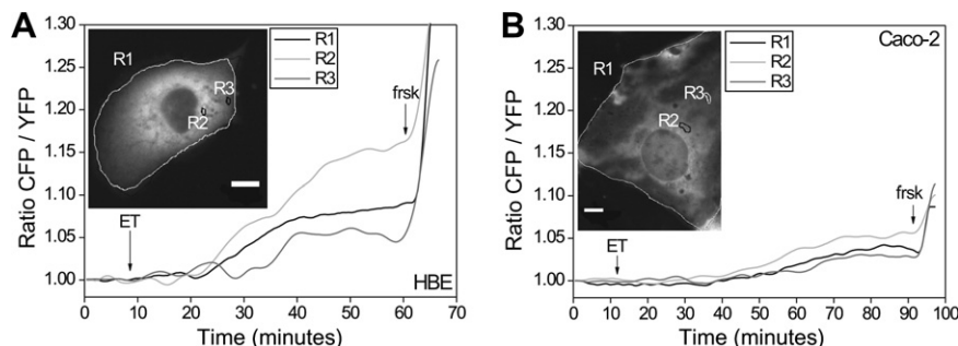
Fig. 4. cAMP imaging in HBE and Caco-2 cells transfected with PKA-based fluorescent probes and treated with the anthrax edema toxin (ET). Caco-2 cells are poorly reactive to the addition of protective antigen (PA, 20 nM) and of edema factor (EF, 10 nM). PA mediates the entry of EF which is an AC causing a modest rise of cAMP in Caco-2 cells, while it is active in HBE cells. Notice that this toxin causes the formation of a gradient of cAMP concentration, higher around the nucleus and lower toward the cell periphery. Bars, 10 \mu m.
