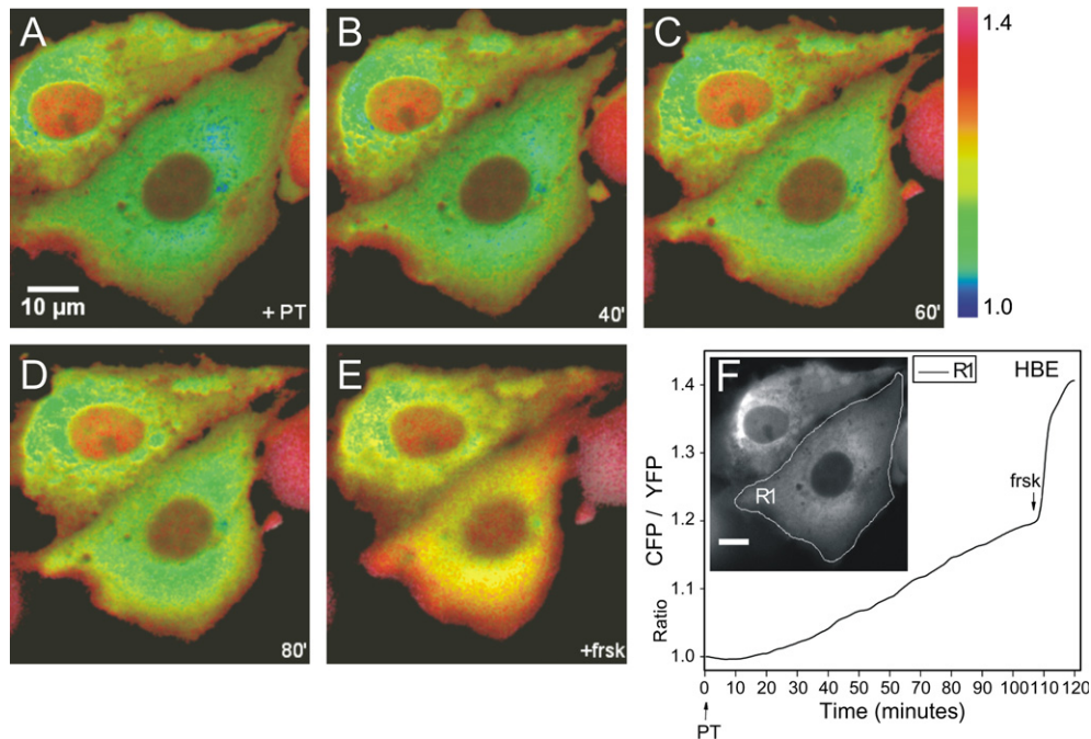
Fig. 1. Imaging of the rise of cAMP induced by pertussis toxin in HBE pulmonary cells transfected with PKA-based fluorescent probes. HBE cells expressing the catalytic PKA subunit-YFP and the regulatory PKA subunit-CFP in the cytosol were imaged after treatment with PT (20 nM). Cells were kept in a micro-incubator at 37 °C and constant 5% CO 2 pressure, under the microscope objective. (A–D) Two cells at the given time periods after toxin addition: the pseudo-colors reflect the increasing cAMP concentration from blue (low cAMP) to red (high cAMP). (E) Effect of the addition of forskolin. (F) Change of cAMP as ratioed in the encircled sub-area indicated in the inset, measured as CFP/YFP ratio. Bars: 10 µm. (For interpretation of the references to color in this figure legend, the reader is referred to the web version of this paper.)
