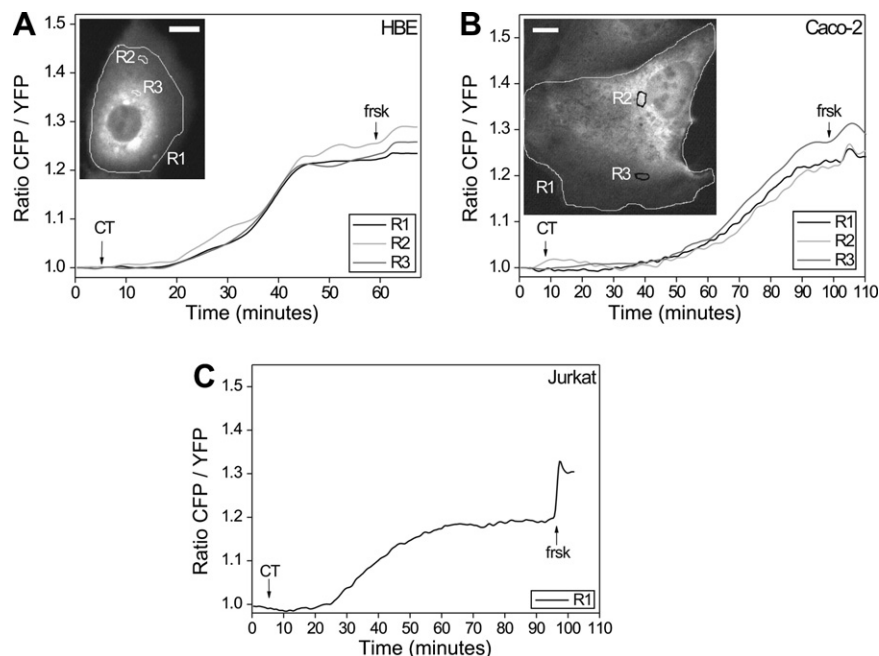
Fig. 3. Time courses of the rise of cAMP as imaged with PKA-based fluorescent probes in HBE, Caco-2 and Jurkat cells treated with cholera toxin (CT). The three cell lines were transfected and imaged as in Figs. 1 and 2, after the exposure to 5 nM CT. The three panels show that all the three cell lines are reactive to CT and that this toxin induces a consistent increase in cAMP cytosolic concentration which begins to rise earlier in Jurkat and HBE than in Caco-2 cells. Bars: 10 \mu m.
