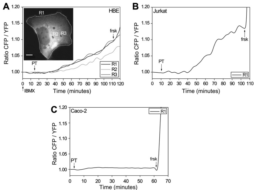
Fig. 2. Time courses of the rise of cAMP as imaged with PKA-based fluorescent probes in HBE, Jurkat cells and Caco-2 treated with pertussis toxin (PT). The three panels show traces of the increase of cytosolic cAMP as detected with the method outlined in Fig. 1 in the indicated cell lines treated with 20 nM PT. (B) Record obtained monitoring the entire cell area, given the reduced dimension of the cytosol of the Jurkat T cells, while three different sub-areas are monitored in the larger HBE cell. The increase in cAMP in the Jurkat T cells and in the pulmonary HBE cells is low, as compared to other toxins (see Figs. 3 and 4), but it is clearly evident after a lag phase of 30–40 min; this gives an in vivo indication of the time required for PT to traffic its S1 ADP-ribosyltransferase subunit into the cytosol. In contrast, Caco-2 cells do not rise their cAMP level following the action of PT, though the cells are fully responsive as one can see from the effect of the adenylate cyclase agonist forskolin (abbreviated frsk in A). Bars: 10 µm.
