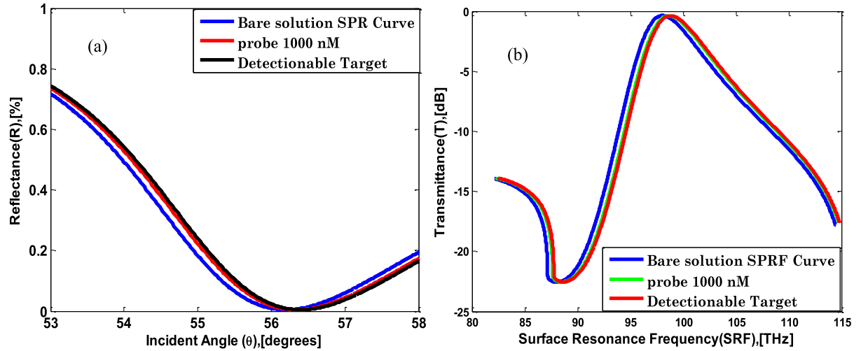
Fig. 2. Numerical results of Bare SPR Sensor (a) R \sim \text{SPR-angle} curve in the absence of formalin and chitosan. (b) T \sim \text{SPRF} curve in the absence of formalin and chitosan.
