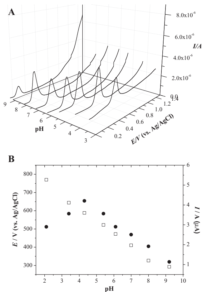
Fig. 3. (A) 3D plots of base-line corrected DP voltammograms obtained in 200 \mu M IDA; (B) plot E_{pa} vs. pH ( \square ) and I_{pa} vs. pH ( \bullet ) of peak 1 a .
