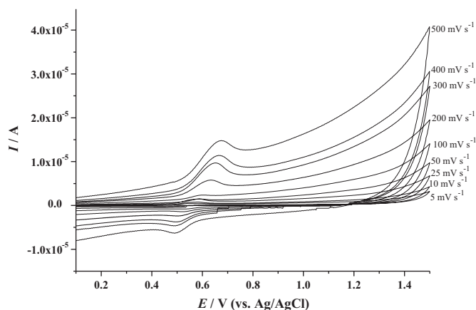
Fig. 2. Cyclic voltammograms of 200 \mu\text{M} IDA in pH = 4.3 0.1 M acetate buffer solution, at different scan rates.
