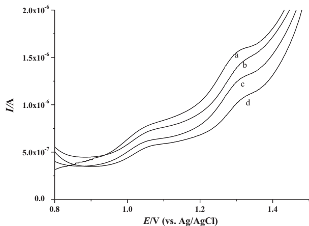
Fig. 4. DP voltammograms obtained in pH = 4.5 0.1 M acetate buffer with ds-DNA biosensors (a) before and after incubation during (b) 5, (c) 10 and (d) 15 min in a solution of 100 \mu M IDA.
