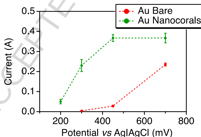
Fig. 3. Effect of the applied potential on the response to 20 \mu M H 2 O 2 obtained for Au bare (red) and Au nanocoral (green). Experiment carried out in 0.01 M PBS solution pH 7.4.
