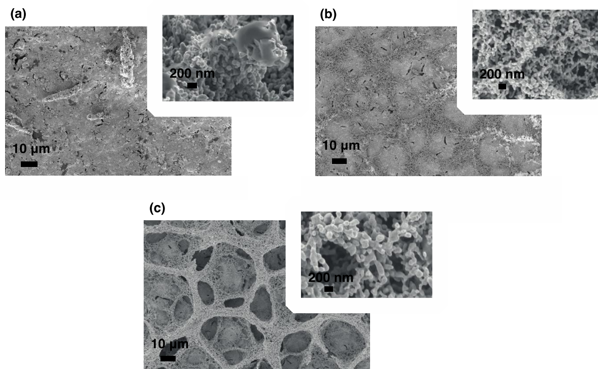
Fig. 1. SEM images of porous gold nanocoral-like structures deposited at -3.0 V for 15 s (a), 60 s (b) and 120 s (c) in a solution of 0.01 M \text{HAuCl}_4 and 2.5 M \text{NH}_4\text{Cl} . Insets show the respective magnifications.
