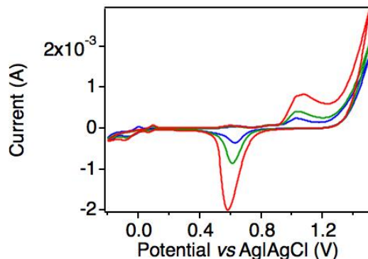
Fig. 2. (a) CVs registered in 0.1 M H 2 SO 4 at 100 mV/s for Au deposited at -3.0 V for 15 s (blue), 60 s (green) and 120 s (red) at a scan rate of 100 mV s -1 .
