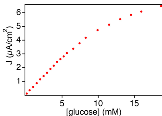
Fig. 6. Current density as a function of concentration of glucose. The amperometric response was obtained to successive addition of glucose in a stirred 10 ml PBS pH 7.4 containing a physiological concentration of NaCl (0.12 M) at +0.15 V (vs Ag/AgCl) using a nanocoral Au based electrode.
