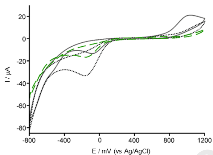
Figure 4. Cyclic voltammograms of [\text{CHI}^{(+)}\text{IL}^{(+)}|\text{CuPc}^{\text{S}(-)}]_2 (____), [\text{CHI}^{(+)}\text{IL}^{(+)}|\text{CuPc}^{\text{S}(-)}]_2|\text{Lac} (.....), and [\text{CHI}^{(+)}\text{IL}^{(+)}|\text{CuPc}^{\text{S}(-)}]_2|\text{CHI}^{(+)}\text{IL}^{(+)}|\text{Lac} (- - -) immersed in 10^{-4} M catechol in 0.01 M phosphate buffer (pH 7.00). Scan rate 100 \text{ mV.s}^{-1} .
