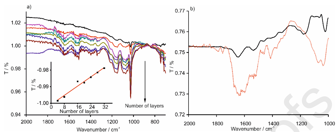
Figure 2. a) FTIR spectra of LbL [CHI(+)+IL(+)|CuPcS(-)] n films with increasing number of layers (n = 4,8,12,16,20,24,28,32). The inset shows the correlation between the transmittance measured at 1027 cm -1 and the number of layers. b) Comparison of the spectra of [CHI(+)+IL(+)|CuPcS(-)] 16 (solid line) and of [CHI(+)+IL(+)|CuPcS(-)] 16 |Lac (dotted line).
