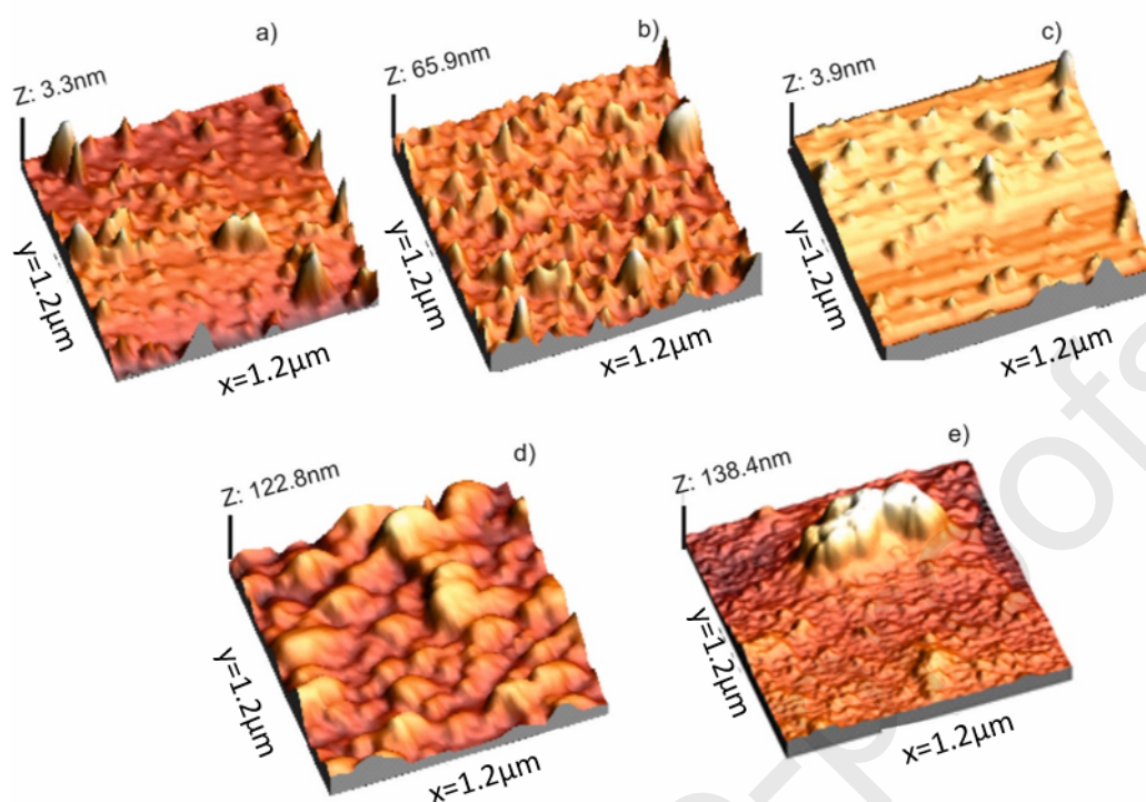
Figure 3. AFM topographic images of a) [\text{CHI}^{(+)} + \text{IL}^{(+)} | \text{CuPc}^{\text{S}(-)}]_2 ; b) [\text{CHI}^{(+)} + \text{IL}^{(+)} | \text{CuPc}^{\text{S}(-)}]_{12} ; c) [\text{CHI}^{(+)} | \text{CuPc}^{\text{S}(-)} | \text{IL}^{(+)} | \text{CuPc}^{\text{S}(-)}]_2 ; d) [\text{CHI}^{(+)} | \text{CuPc}^{\text{S}(-)} | \text{IL}^{(+)} | \text{CuPc}^{\text{S}(-)}]_{12} and e) [\text{CHI}^{(+)} + \text{IL}^{(+)} | \text{CuPc}^{\text{S}(-)}]_2 \text{Lac} . “Note that the vertical heights of surface features varied from \approx 3 nm (panels a and c) to > 120 nm (panels d and e)”
