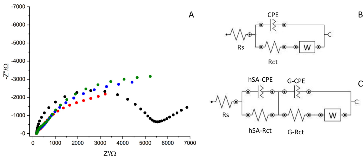
Fig. 3. (A) Nyquist plots for bare (black dots), poly(Py-2-COOH) modified G-SPE (red dots) and hSA poly(Py-2-COOH) modified G-SPE in absence (blue dots) and presence of 1 \mu M PFOA (green dots), (B) modified Randles EEC; (C) hSA modified electrode EEC. All the measurement were performed in 0.1 M KNO_3 with 2 mM [Fe(CN_6)]^{3-/4-} . (For interpretation of the references to colour in this figure legend, the reader is referred to the web version of this article.)
