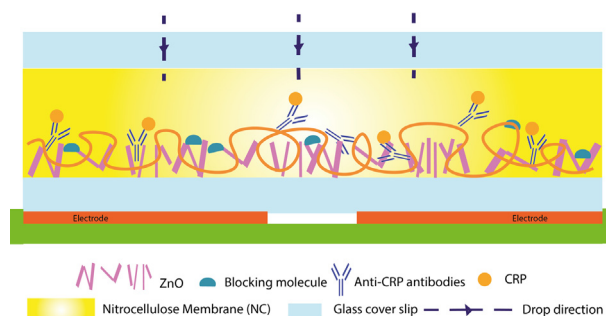
Scheme 2. Illustration of the ZnO nanoparticle nitrocellulose membrane sandwiched between two coverslips positioned above the electrodes.
