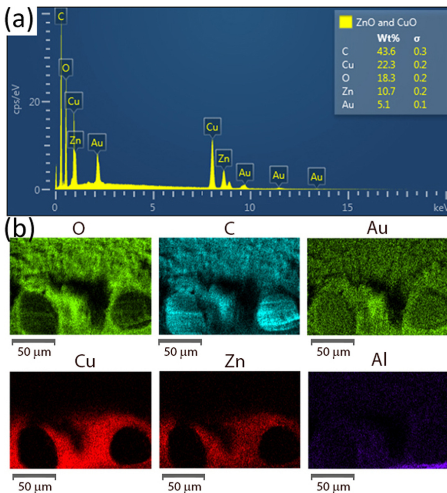
Fig. 4. EDS spectrum/mapping on the lower layer cross-section of the nano-ZnO/CuO membrane: (a) EDS spectrum and (b) EDS mapping of the elements: O, C, Au, Cu, Zn and Al.
