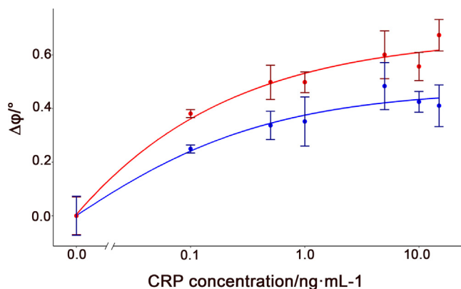
Fig. 7. Phase change/degree ( \Delta\phi/^\circ ) response versus antigen (CRP) concentration for sonicated nano-ZnO nitrocellulose membranes (blue) and nano-ZnO/CuO nitrocellulose membranes (red) with capture antibody ( n = 3 ) measured at the frequency of 100 Hz, - standard error bars are shown. (For interpretation of the references to colour in this figure legend, the reader is referred to the web version of this article.)
