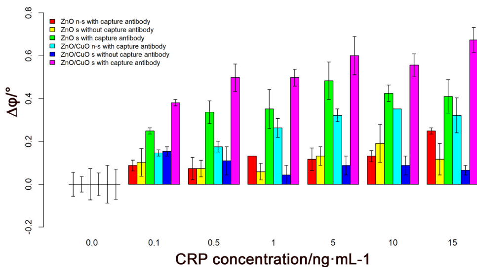
Fig. 6. Impedance phase change/degree ( \Delta\phi/^\circ ) response to seven concentrations of antigen (CRP) on the six different types of membrane. For the 3 nano-ZnO membranes ( n = 3 ): with 200 ng capture antibody and without sonication (red), without capture antibody and with sonication (yellow) and with 200 ng capture antibody and with sonication (green). For the 3 nano-ZnO/CuO membrane ( n = 3 ): with 200 ng capture antibody and without sonication (light blue) and without capture antibody but with sonication (dark blue), with 200 ng capture antibody and with sonication (pink purple). (For interpretation of the references to colour in this figure legend, the reader is referred to the web version of this article.)
