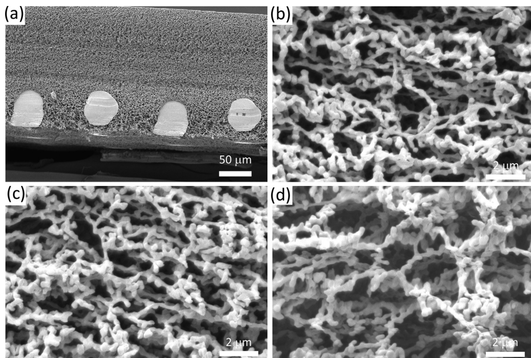
Fig. 1. Scanning electron micrographs of the nitrocellulose membrane cross-section: (a) whole cross section at 1000 \times magnification; (b) upper layer of nano-ZnO/nitrocellulose membrane (with small pore structures) at 30,000 \times magnification; (c) middle layer of nano-ZnO/nitrocellulose membrane (with bigger and loose pore structures) at 30,000 \times magnification; (d) lower layer of nano-ZnO/nitrocellulose membrane (with biggest pore structures) at 30,000 \times magnification.
