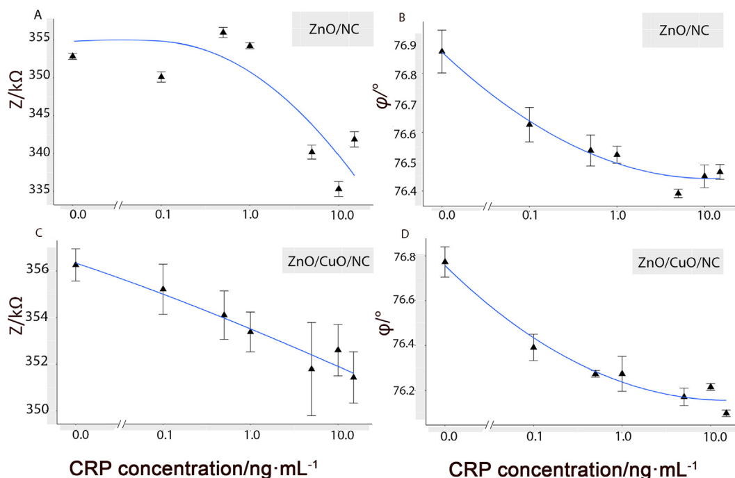
Fig. 5. Impedance amplitude/kOhms ( Z/k\Omega ) and phase change/degree ( \phi/^\circ ) on nano-ZnO nitrocellulose membranes ( n = 3 ) and nano-ZnO/CuO nitrocellulose membranes ( n = 3 ) after a 10-min incubation time with increasing concentrations of CRP, measured at a frequency of 100 Hz.
