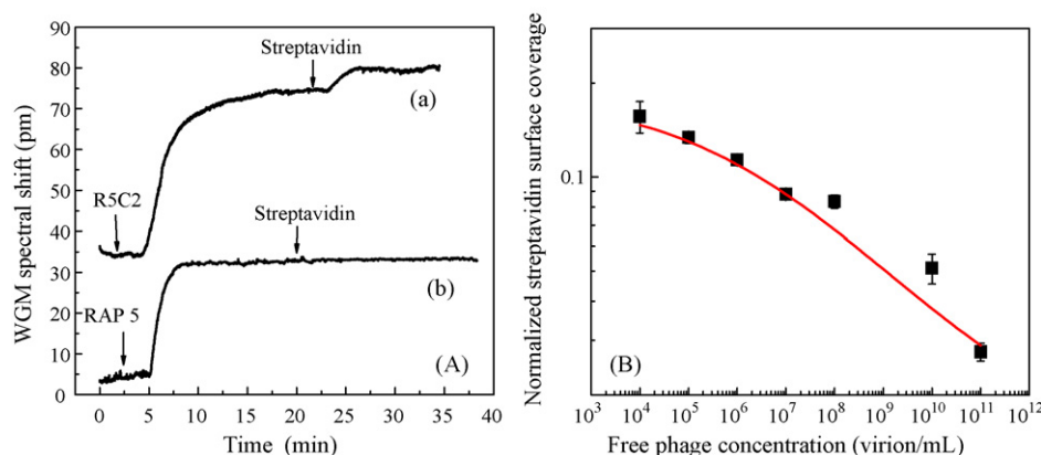
Fig. 4. (A) Sensing specificity test. (a) The OFRR response with working phase R5C2 and (b) the OFRR response with negative control phage RAP 5. (B) Competitive binding assay for phage specificity test. WGM spectral responses to the phage probe on the sensing surface to the streptavidin (1.8 \mu M). Streptavidin was incubated with free phage ( 10^{11} – 10^4 virion/mL) prior to exposure to sensing surface. Each experiment was repeated three times.
