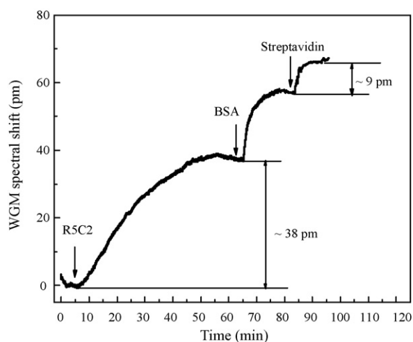
Fig. 3. Sensorgram for streptavidin detection. The interior surface of OFRR was immobilized with working phase probes R5C2, and then the unoccupied sites were blocked with BSA. Finally, the sensing surface was exposed to 1.8 \mu M streptavidin.
