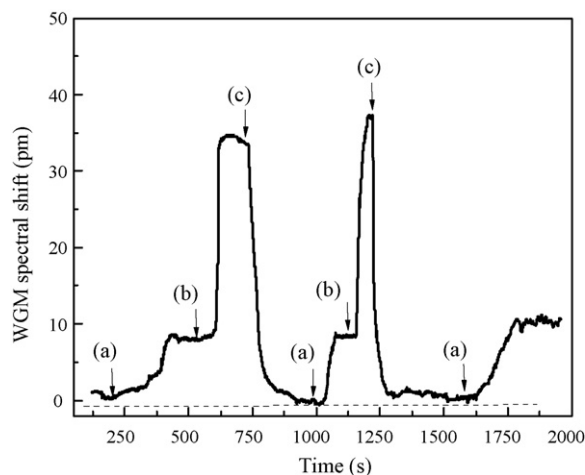
Fig. 6. Sensorgram in response to sensing surface regeneration. (a) Injection of 1.8 \mu M streptavidin that binds to the sensing surface, (b) injection of cocktail regeneration solution to remove streptavidin from the sensing surface and (c) injection of PBS buffer to rinse off the cocktail regeneration solution and re-establish the detection baseline. Dashed line is the sensing baseline.
