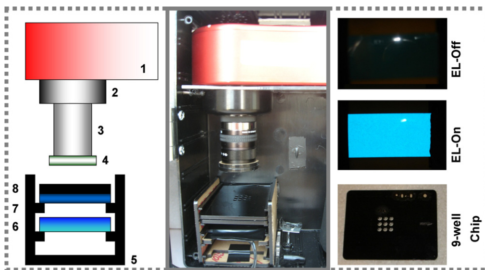
Fig. 1. The EL-CCD point of care detector. (A) A schematic configuration of the detector and (B) a photograph of the actual detection platform where: Atic-16 CCD camera [1] is equipped with one of two green band pass filters. A 5 mm extension tube [2] is attached to the 12 mm Pentax f1.2 lens [3]. The second green band pass filter B [4] is mounted on the end of the lens. A black acrylic shelf box [5] was designed to hold the EL strip panel [6], the blue band pass filter [7] and the black acrylic 9-well sample chips [8]. (C) Photographs of Royal Blue EL strip off and on and the black acrylic 9-well chips designed to hold aqueous samples for imaging. (For interpretation of the references to color in this figure legend, the reader is referred to the web version of the article.)
