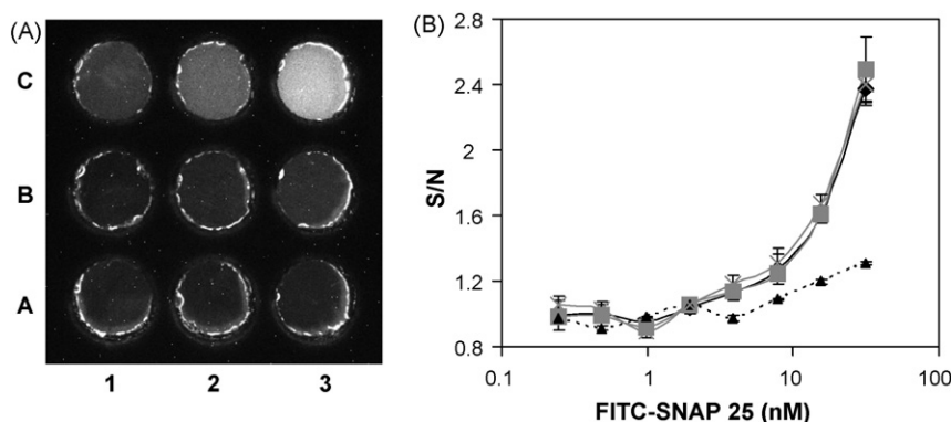
Fig. 2. The optimization of the 9-well chip base material using FITC-SNAP-25 peptide. (A) CCD image of FITC-SNAP-25 dose response solutions added to the 9-well black chip taken using the EL-CCD detector, 120 s exposure. The COC based wells were loaded with FITC-SNAP-25 at concentrations ranging from 0 nM (A1) to 31.25 nM (C3). (B) The dose response curves plotted versus signal-over-noise (therefore blank = 1) for the different chip base materials; COC (black diamonds/solid line), PC (gray squares/solid line), Mylar (black triangles/dashed line) and glass (gray crosses/dashed line). Standard deviations were determined from n \geq 3 chips.
