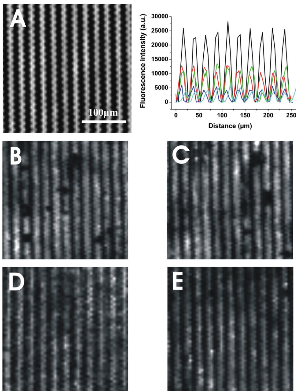
Fig. 3. Fluorescence images of (A) microcontact printed lines of \alpha -hu IgG labelled with DY-636 (A) before and after transfer onto (B) glass and (C) Zeonor ® as a second substrate. Fluorescence images of microcontact printed lines of \alpha -hu IgG after transfer onto (D) glass and (E) Zeonor ® as second substrate, blocking with BSA and incubated with hu-IgG labelled with DY-636. Graph (top right): section analysis of fluorescence intensity perpendicular to: microcontact printed lines of hu-IgG labelled with DY-636 before transfer (black); microcontact printed lines of hu-IgG labelled with DY-636 after transfer onto glass (red) and Zeonor ® (green) as second substrate; microcontact printed lines of \alpha -hu IgG after transfer onto a glass (dark blue) and Zeonor ® (light blue) as a second substrate, blocking with BSA and incubation with hu-IgG labelled with DY-636. (For interpretation of the references to color in this figure legend, the reader is referred to the web version of the article.)
