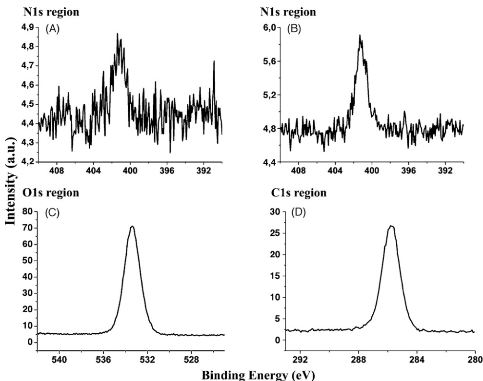
Fig. 1. XPS spectra at different stages of the transfer process: (A) N1s region after hu-IgG deposition on silicon, (B) N1s region after trehalose deposition on hu-IgG on silicon, (C) O1s and (D) C1s region after PECVD deposition of HMDSO on trehalose on hu-IgG on silicon.
