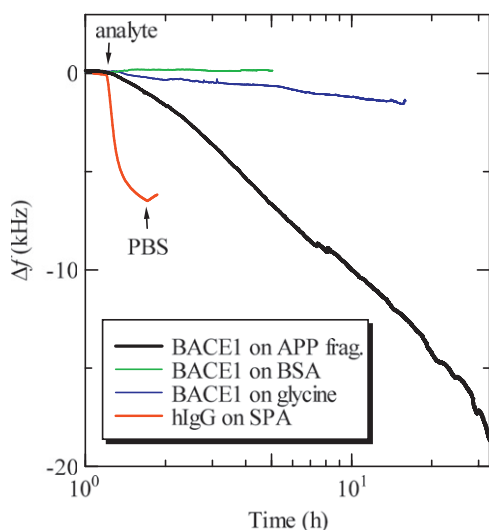
Fig. 1. Frequency changes during various binding reactions: 5 \mu g/ml BACE1 on APP fragment (Black), BSA (green), and glycine (blue); and 10 \mu g/ml hIgG on SPA (red). Note that a logarithmic time scale is used. (For interpretation of the references to color in this figure caption, the reader is referred to the web version of this article.)
