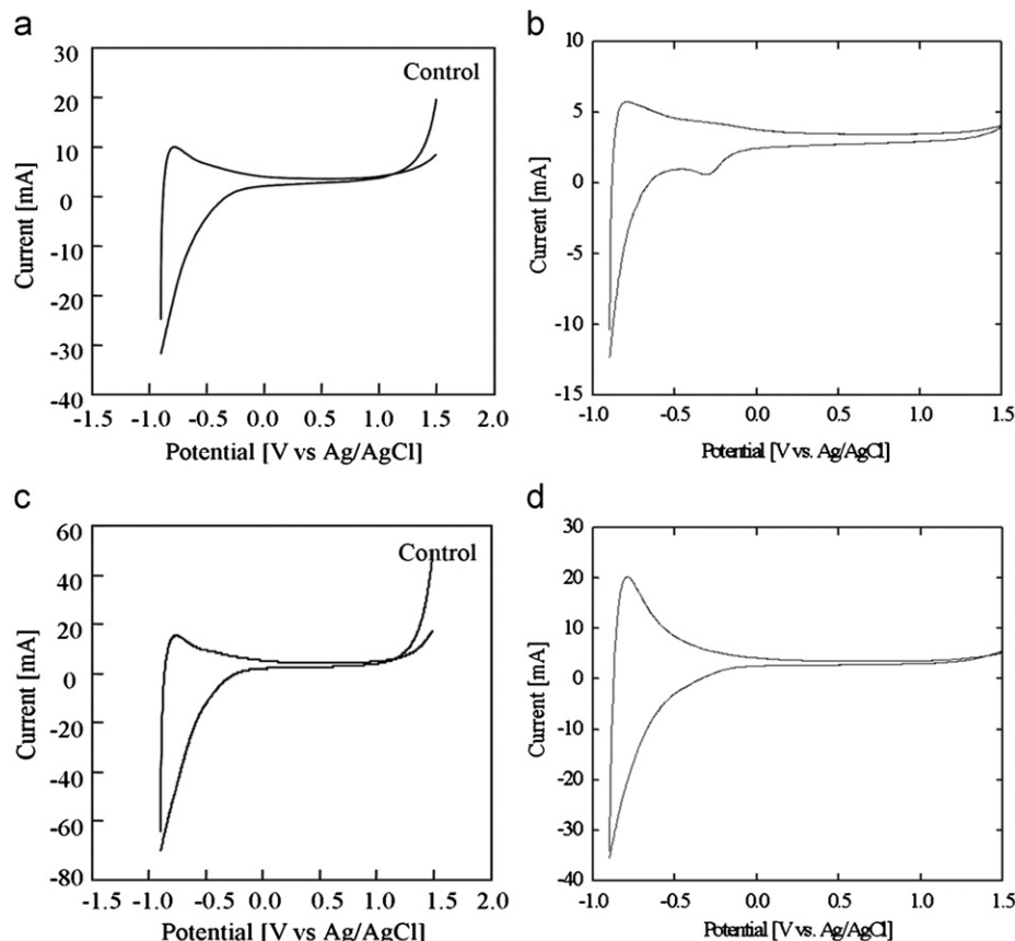
Fig. 3. CV of 35 nm reaction site electrode (a), HRP-immobilized 35 nm reaction site electrode (b), 200 nm reaction site electrode (c), and HRP-immobilized 200 nm reaction site electrode (d).
