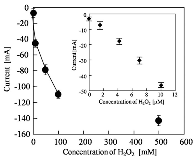
Fig. 5. Calibration plot for the fabricated HRP/nTOFs/Ti-biosensors having 70 nm diameter reaction site at -0.35 \text{ V} .
