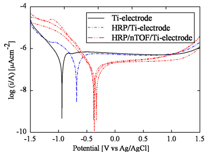
Fig. 2. Tafel plots of Ti-, HRP/Ti-, and HRP/nTOFs/Ti-electrodes. HRP/nTOFs/Ti-electrodes were fabricated by three different surfaces which are treated by various concentrations of KOH aqueous solution (1.0, 15 and 25 mol/L).
