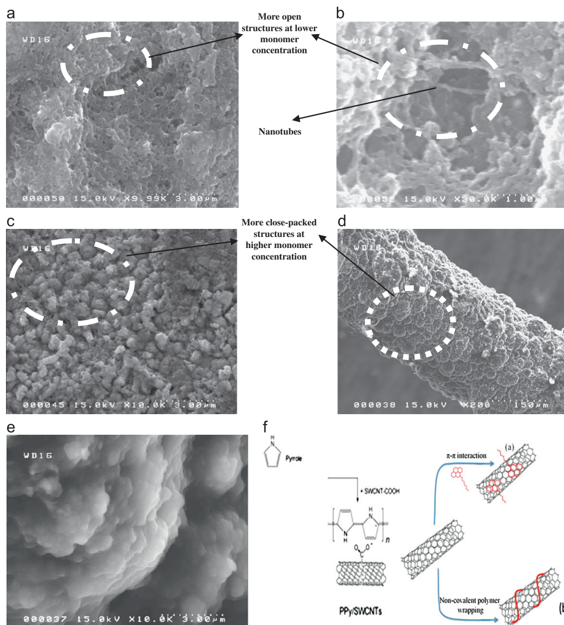
Fig. 1. (a) and (b) SEM images of SWCNT/Au/PPy-GOx assembled with 0.05 M pyrrole. (c) SEM image of SWCNT/Au/PPy-GOx assembled with 0.1 M pyrrole. (d) SEM image of SWCNT/Au/PPy-GOx assembled with 0.5 M. (e) A micrograph of a zoom of a particular area, of the same sample. (f) A cartoon of the mechanism of the polymer entrapments into the SWCNTs.
