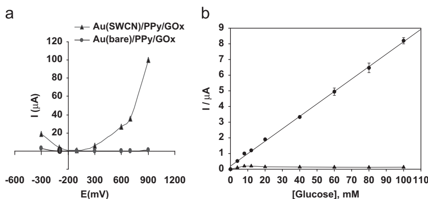
Fig. 2. (a) Hydrodynamic Voltammograms (HDV) for 4 mM glucose recorded at the Au/SWCN/PPy-GOx microelectrodes (▲), and at the Au(bare)/PPy-GOx microelectrodes (●). (b) Calibration plot for glucose (●) having the response linearity ranging from 4 to 100 mM glucose with a CV% of 2. Flat line (▲) corresponds to the 0.1 mM acetaminophen. No signal was detected for AA and UA.
