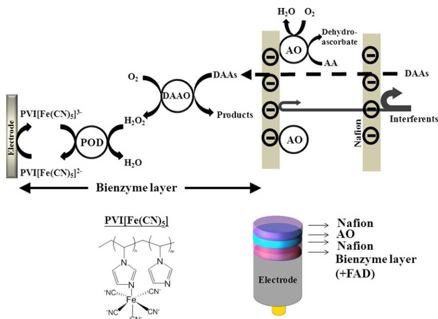
Scheme 2. The composition and the reaction sequence of the proposed DAAO/POD bienzyme biosensor protected by Nafion and AO.
