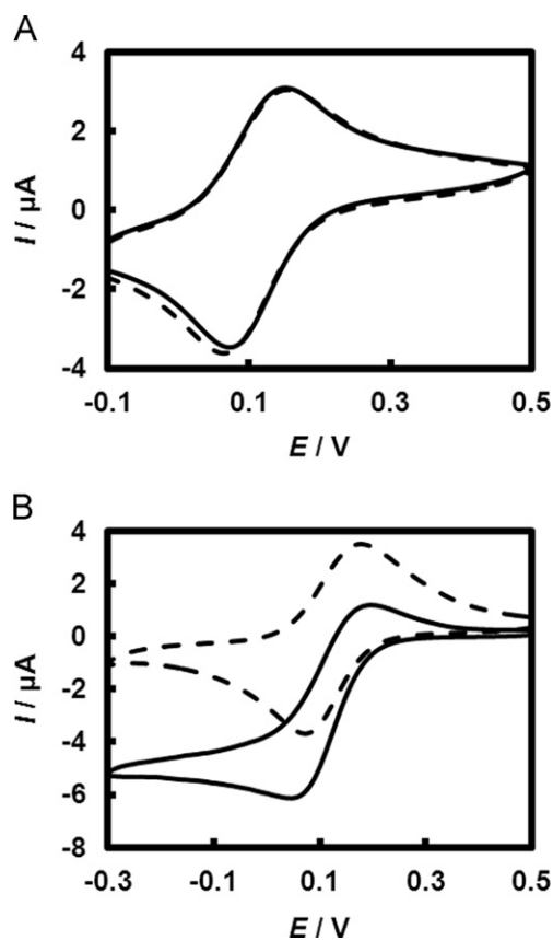
Fig. 1. Cyclic voltammograms of (A) DAAO/PVI[Fe(CN) 5 ]-modified electrode in an Ar-saturated solution and (B) DAAO/POD/PVI[Fe(CN) 5 ]-modified electrode in an Air-saturated solution. The dashed line is the detection in a buffer solution and the solid line is the detection in 4 mM D-alanine (pH 8.0). Electrode composition, DAAO: 0.33 U, POD: 2.14 U, PEGDGE: 10 μg, PVI[Fe(CN) 5 ]: 20 μg. Scan rate is 20 mV s -1 .
