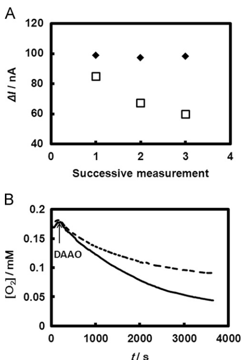
Fig. 2. Dependence of the current response at -0.1 V on the successive measurements in the solution containing 40 \mu\text{M} FAD and 5 \mu\text{M} D-alanine (closed rhombus) or 5 \mu\text{M} D-alanine only (open square). Electrode composition, DAAO: 0.25 U, POD: 2.67 U, PEGDGE: 10 \mu\text{g} , PVI[Fe(CN) _5 ]: 30 \mu\text{g} . (B) Time dependence of the dissolved oxygen concentration during the DAAO reaction in the solution containing 40 \mu\text{M} FAD and 4 mM D-alanine (solid line) or 4 mM D-alanine only (dashed line).
