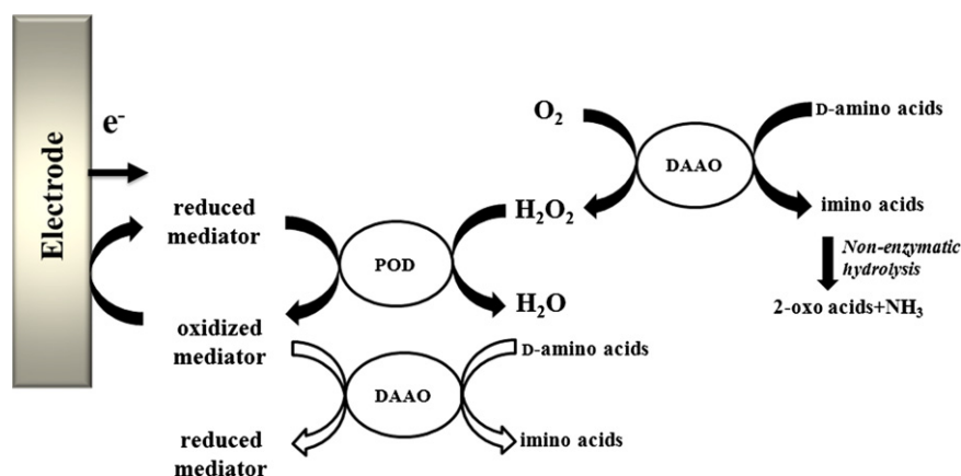
Scheme 1. Possible reactions in mediated DAAO/POD bienzyme sensor.
