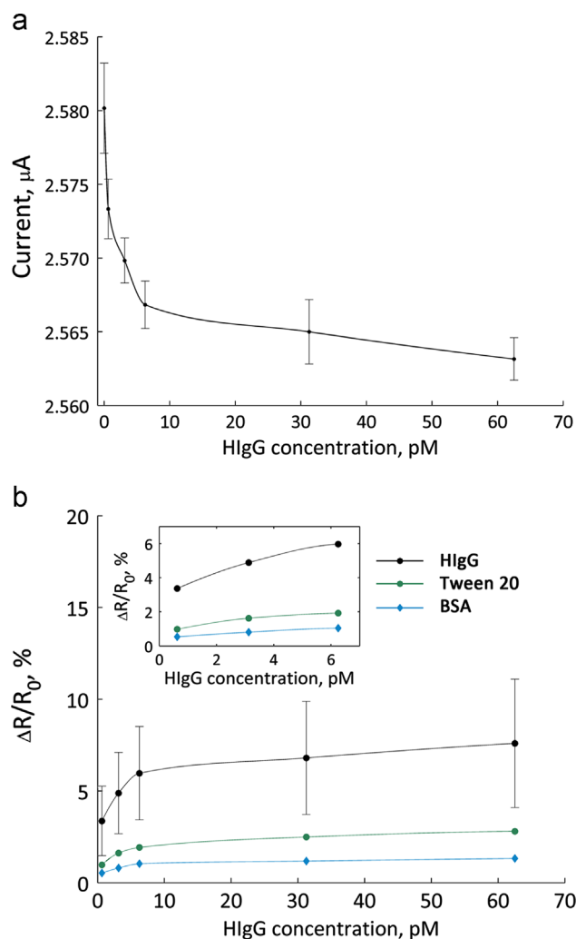
Fig. 3. (a) Response of one biosensor in 2 mM PBS. Each data point is an average of three measurements with the same sensor. The error bars correspond to the standard deviations of the three measurements. (b) Biosensor calibration for HlgG in 2 mM PBS (black; upper curve), negative control with BSA (blue; bottom curve), and the Tween 20 control experiment where no antibody was immobilized onto SWCNTs control (green; middle curve). Data points of HlgG calibration are averages of three different biosensors with the corresponding standard deviation. The inset shows a magnification (without error bars) of the low concentration range. (For interpretation of the references to color in this figure legend, the reader is referred to the web version of this article.)
