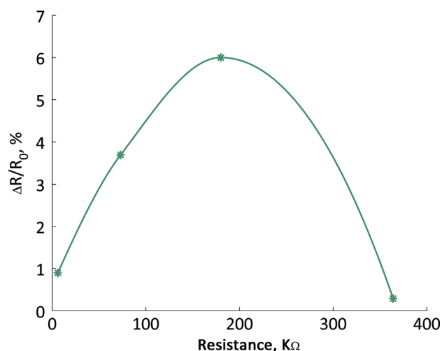
Fig. 2. Dependence of the instrumental response on the resistance of the paper-based chemiresistor for 6.3 pmols · L -1 of HlgG. The plot was adjusted using a spline curve.
