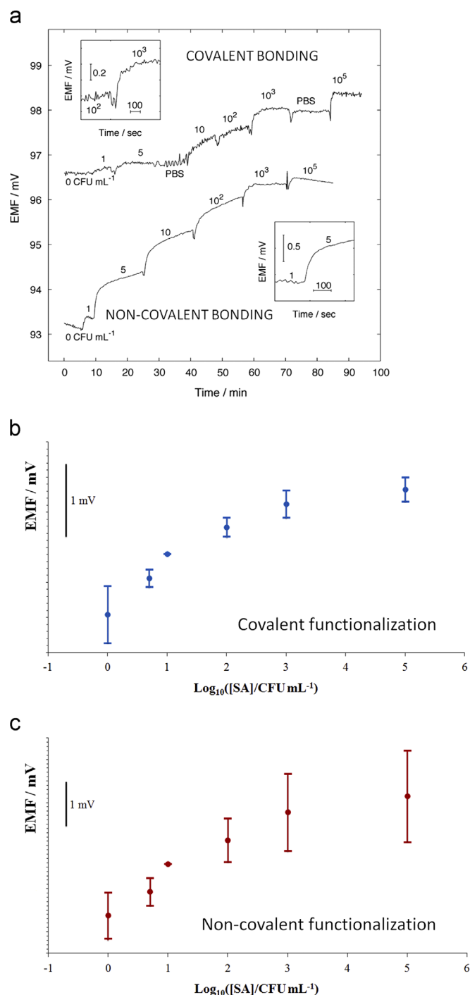
Fig. 2. (a) Aptamer-functionalized aptasensor exposed to stepwise increases of S. aureus concentration and the corresponding potentiometric response; numbers above each potentiometric jump represent the final concentration of bacteria. Insets show the detail of two inoculation steps for the covalent and non-covalent functionalization. (b) EMF response versus log of concentration of S. aureus for the covalent functionalization. (c) EMF response versus log of concentration of S. aureus for the non-covalent functionalization. In (b) and (c) error bars are standard deviation of the response obtained at a given concentration for six different sensors. The sensitivities of the aptasensors are 0.34 mV/decade (covalent functionalization) and 0.55 mV/decade (non-covalent functionalization).
