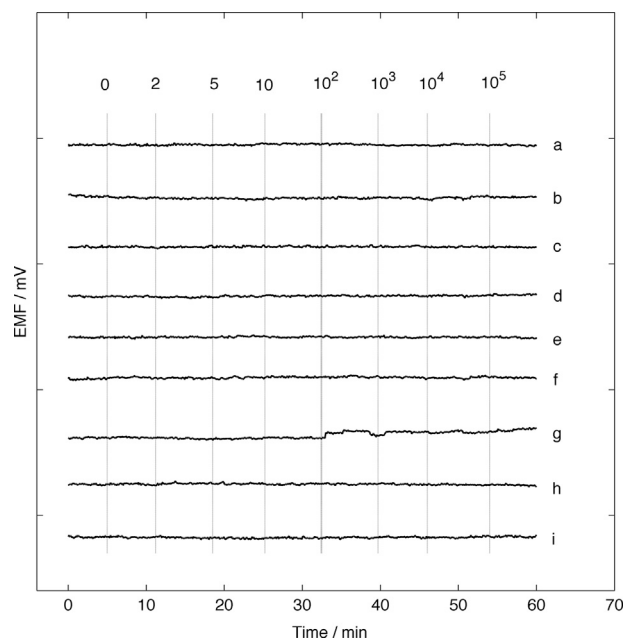
Fig. 3. Selectivity ((a)–(d)) and control ((e)–(i)) assays. EMF response versus time for different concentrations of bacteria. Vertical lines represent inoculation with increasing amounts of bacteria (in CFU/mL). From top to bottom: (a) and (b) Covalently functionalized biosensor exposed to Escherichia coli and L. casei , respectively; (c) and (d) Non-covalently functionalized biosensor exposed to E. coli and L. casei , respectively; (e) Glassy carbon electrode exposed to S. aureus ; (f) and (g) Glassy carbon without GO/RGO covalently and non-covalently functionalized with aptamer exposed to S. aureus ; (h) Glassy carbon with a layer of GO/RGO and without aptamer exposed to S. aureus ; (i) Non-covalently functionalized aptasensor without pyrenil moieties in the aptamer exposed to S. aureus .
