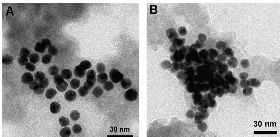
Fig. 4. TEM images of (A) 4.9 nM AuNPs–10 nM TBA–10 nM PDDA, and (B) 4.9 nM AuNPs–10 nM TBA–1 \mu\text{M} thrombin–10 nM PDDA.
