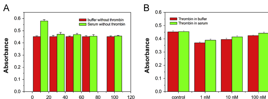
Fig. 6. Results obtained from the testing of (A) Tris-HCl buffer solution and serum samples with different dilution ratios without thrombin, and (B) 70-fold diluted serum samples spiked with different concentrations of thrombin.
