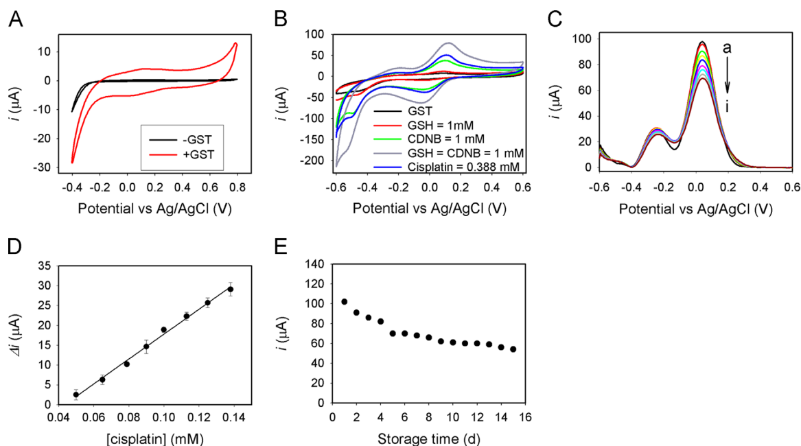
Fig. 3. (A) CV of carbon paste electrode unmodified and modified with GST at potential between -0.4 and 0.8 V. Supporting electrolyte was 50 mM PBS (pH 6.5); scan rate = 0.1 V/s. (B) CV of carbon paste electrode modified with GST showing response of the substrates and the inhibition effect of cisplatin. With GSH, the enzyme modified electrode shows a small increase in current, which is attributed to the redox reaction of GSH to GSSG (red or the second lowest line). When CDNB is added without GSH, a stronger signal is observed (green or the third lowest line). This is attributed to the reaction of CDNB with the electrode. When GSH and CDNB are added together, a large increase in current is observed (gray or the highest line) since both substrates of GST are present. As GSH being consumed, the conversion from GSSG to GSH becomes more efficient. Finally, when the inhibitor (cisplatin) is introduced to compete with the substrate, a decrease of the current is observed (blue or the next to the highest line). (C) SWV spectra under optimized conditions: 50 mM phosphate buffer (pH 6.5) with increasing cisplatin concentrations. [GSH] = [CDNB] = 1 mM, [cisplatin] in mM: a=0 ; b=0.05 ; c=0.065 ; d=0.079 ; e=0.09 ; f=0.10 ; g=0.11 ; h=0.12 ; i=0.14 . (D) Quantification of the peak current drop as a function of cisplatin concentration, n=4 ; RSD = 4.2\% . (E) Stability of GST enzyme electrode in the electrochemistry measurements over 15 days.
