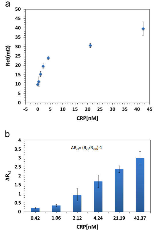
Fig. 4. Recorded ' R_{\text{ct}} ' values and respective change in charge transfer resistance ' \Delta R_{\text{ct}} '; (a) ' R_{\text{ct}} ' vs. different concentrations of CRP on anti-CRP immobilized device, (b) change in ' R_{\text{ct}0} ' (charge transfer resistance for anti-CRP) with respect to different CRP concentrations.
