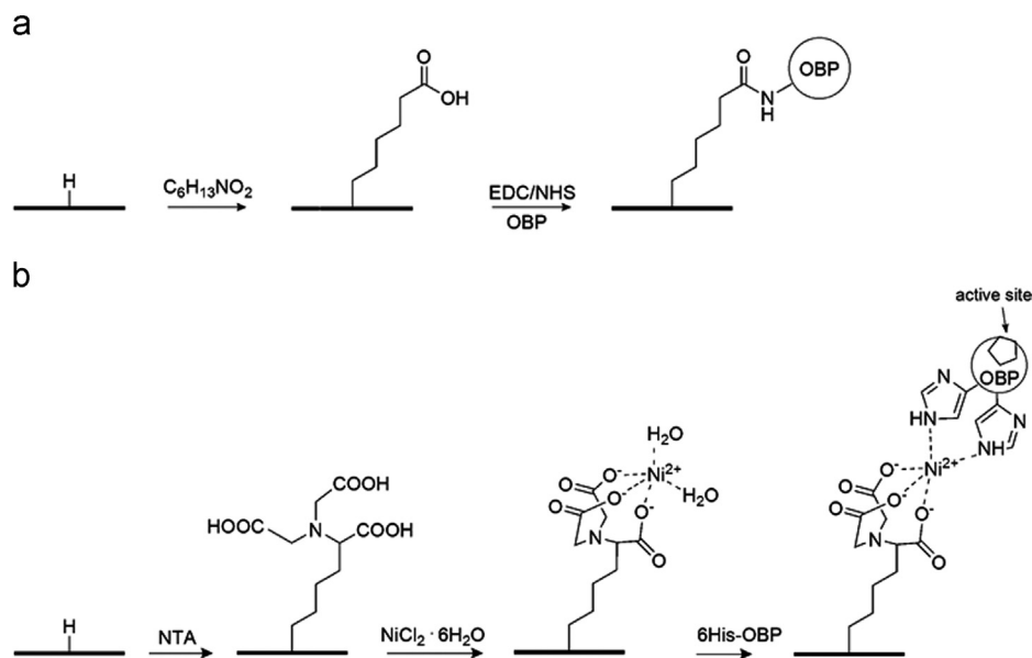
Fig. 1. Summary of OBP immobilization on hydrogenated diamond surfaces using grafting method (1), (a) and using grafting method (2), (b).
