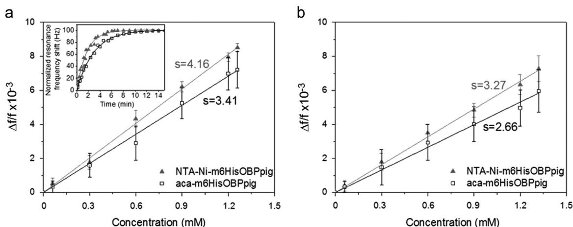
Fig. 5. Concentration response profile for NTA-Ni-m6HisOBPpig and aca-m6HisOBPpig based biosensors (a) upon exposure to different concentrations of IBMP; inset: kinetics response curves upon a specific concentration of IBMP; (b) upon exposure to different concentrations of 2,4-DNT. Errors bars: \pm Standard deviation (SD) calculated from 5 measurements carried out on 5 cantilevers.
