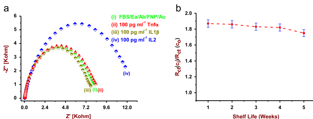
Fig. 6. (a) Nyquist plots of FBS/EA/anti-IL2/FNP/Au electrode in (i) buffer only, (ii) after incubation with 100 \text{ pg ml}^{-1} of \text{TNF-}\alpha , (iii) after incubation with 100 \text{ pg ml}^{-1} of IL1 \beta and (iv) after incubation with 100 \text{ pg ml}^{-1} of IL2. (b) Shelf-life study of FBS/EA/anti-IL2/FNP/Au electrode using 100 \text{ pg ml}^{-1} concentration.
