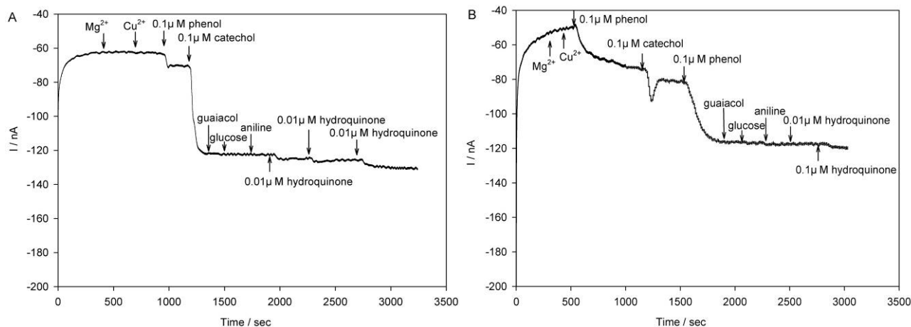
Fig. 4. (A) Current-time response curves of GCE/MCN/Tyr with addition of different interfering substance under the optimized experimental conditions of catechol (pH 6.98, applied potential -0.0664 V). (B) Current-time response curve of GCE/MCN/Tyr with addition of different interfering substance under the optimized experimental conditions of phenol (pH 6.98, applied potential -0.0205 V).
