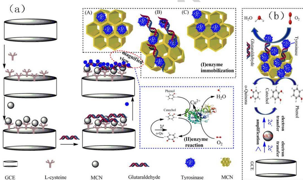
Scheme. 1. Schematic illustration of the tyrosinase biosensor preparation and the proposed mechanism for the phenol and catechol electrocatalytic detection (a). Signal transduction and amplification mechanism of biosensor (b).
