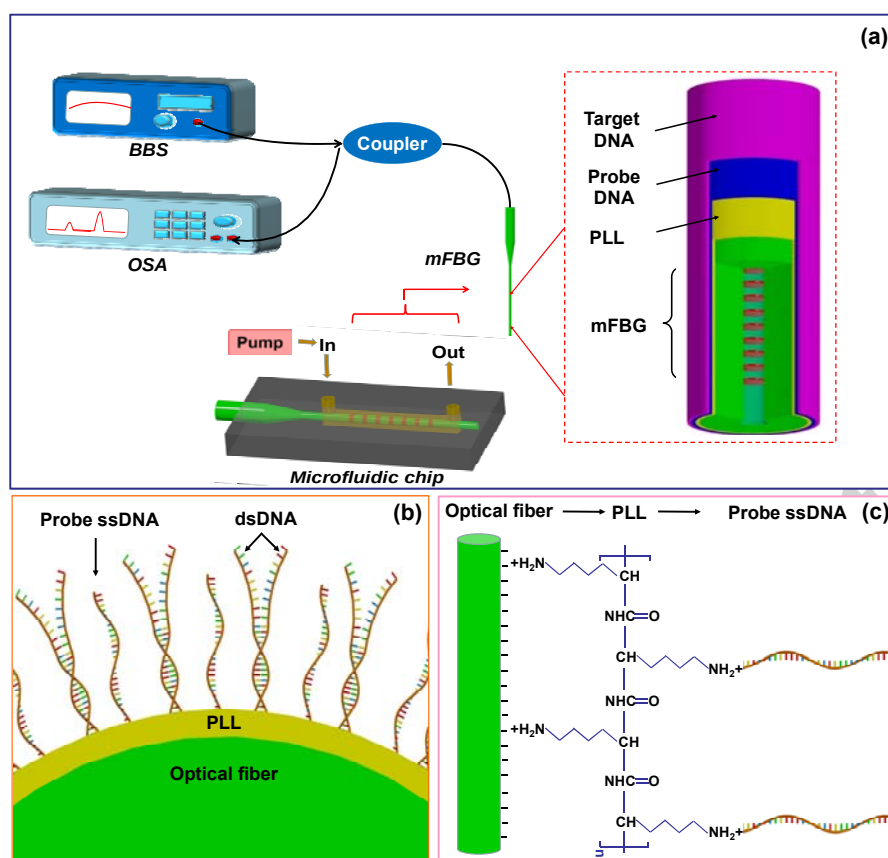
Fig. 5. (a) The schematic of the optical setup of mFBG biosensor (Inset zooms in the configuration of the sensor probe and the microfluidic chip), (b) the scheme of surface functionalization of mFBG biosensor, and (c) the sandwich-like probe system used for target DNA detection.
