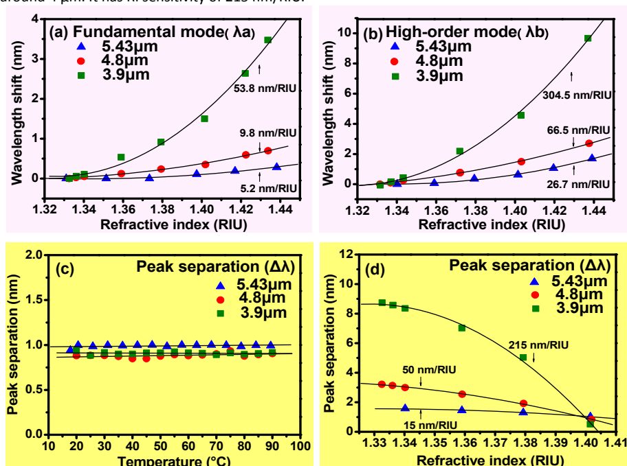
Fig. 2. Relationships between peak wavelength shift and RI of mFBGs with different diameters: (a) fundamental mode ( \lambda_a ) and (b) high-order mode ( \lambda_b ), wavelength separation ( \Delta\lambda=\lambda_a-\lambda_b ) response to (c) temperature fluctuations and (d) RI, respectively.
