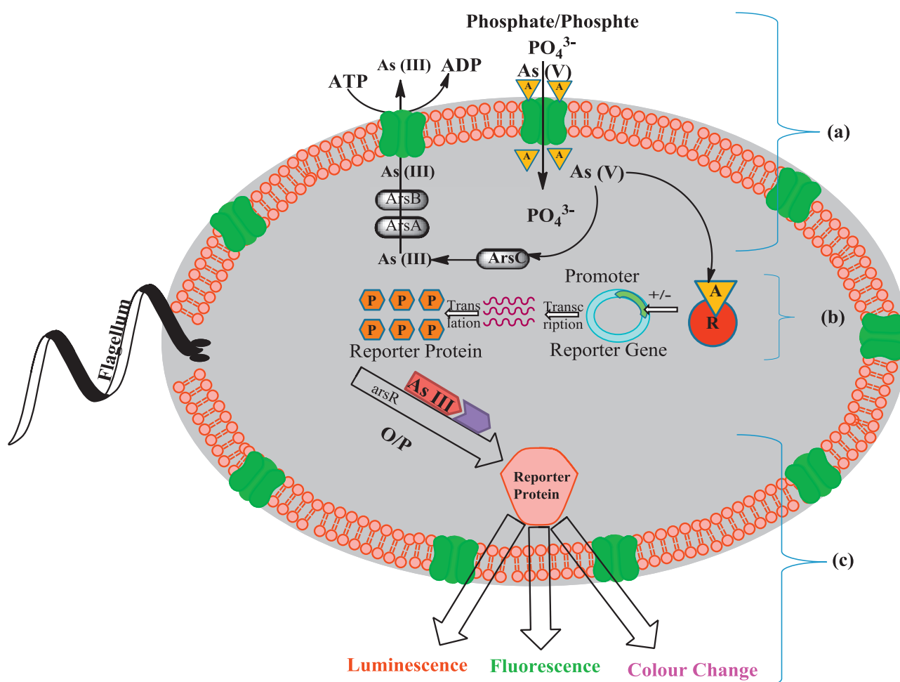
Scheme 2. Schematic representation of whole-cell-based biosensor for (a) Arsenic [As(V) and As(III)] transport by phosphate channel (b) Working mechanism of signal transducer for arsenic biosensor, and (c) Detection of As(III) by luminescence, fluorescence and color change. (For interpretation of the references to color in this scheme legend, the reader is referred to the web version of this article.)
