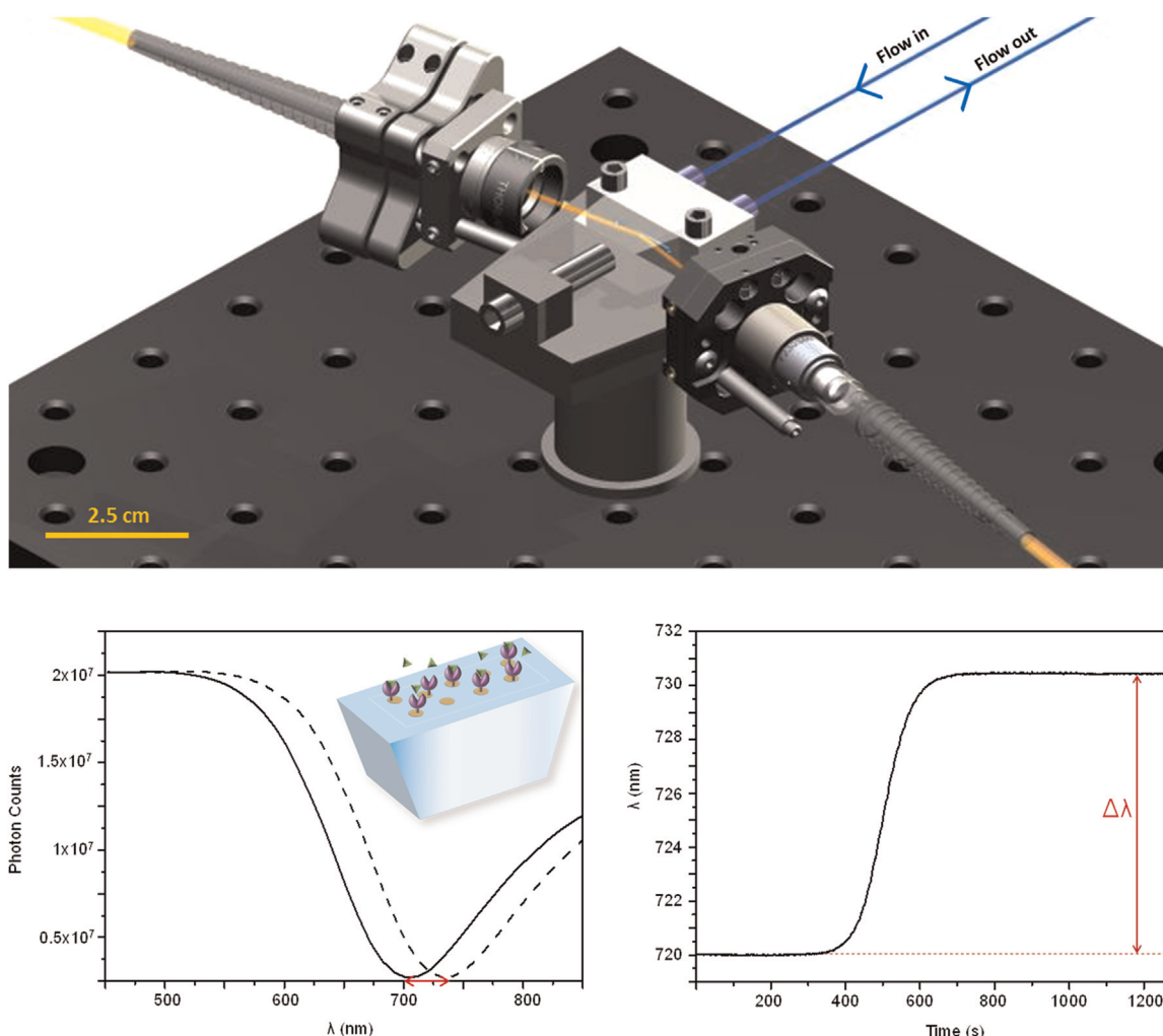
Fig. 1. Top: Schematic of the miniaturized nanoplasmonic biosensor. Bottom: (left) graph showing the resonance peak (photon counts vs. \lambda ); (right) graph showing the shift of the resonance peak over time ( \Delta\lambda_{\text{LSPR}} of the minimum vs. time).
