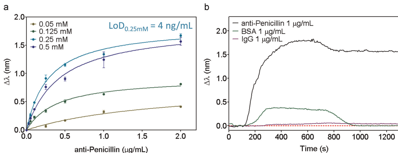
Fig. 3. (a) Calibration curves for anti-penicillin detection at different d-BAPADG2-AXO concentrations (0.05–0.5 mM) performed with 80°-nanoplasmonic sensor; (b) specificity study for the d-BAPADG2-AXO based strategy: sensorgrams for the detection of specific anti-penicillin antibody (black), nonspecific IgG antibody (purple) and bovine serum albumin (green) at 1 \mu\text{g/mL} ; red dashed line indicates reference (background signal). Assays performed with 80°-nanoplasmonic setup. (For interpretation of the references to color in this figure legend, the reader is referred to the web version of this article.).
