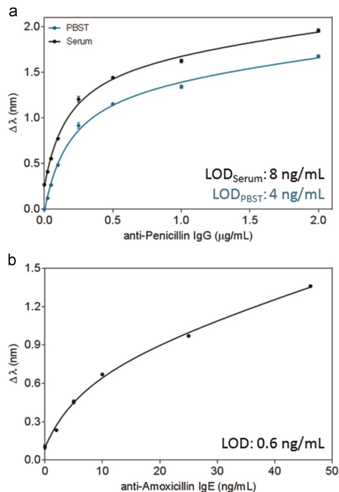
Fig. 5. (a) Anti-penicillin IgG calibration curves in PBST (blue) and whole serum (black); (b) amoxicillin-specific IgE calibration curve in serum samples. (For interpretation of the references to color in this figure legend, the reader is referred to the web version of this article.)
