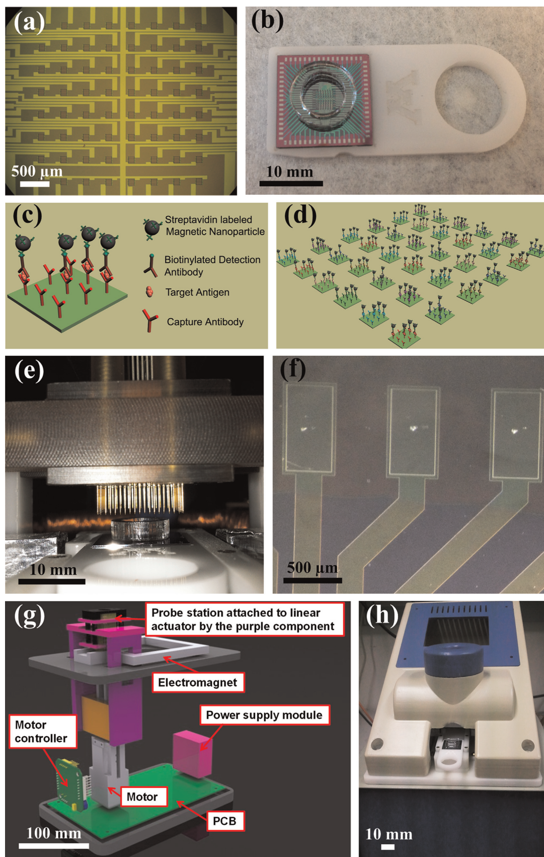
Fig. 1. (a) Photograph of the 64 ( 8 \times 8 ) array) sensors on one chip. (b) Photograph of one GMR chip with the size of 16 mm \times 16 mm and one reaction-well attached chip on the chip holder. (c) Schematic representation of sandwich assay on one GMR sensor. (d) Schematic drawing of the multiplex protein array on one chip. (e) Photograph of Pin array aligning and moving close with the electrode pads of the GMR chip. (f) The marks made by compressed pins on electrode pads. (g) Schematic design of the probe station. (h) Photograph of lab-based probe station system.
