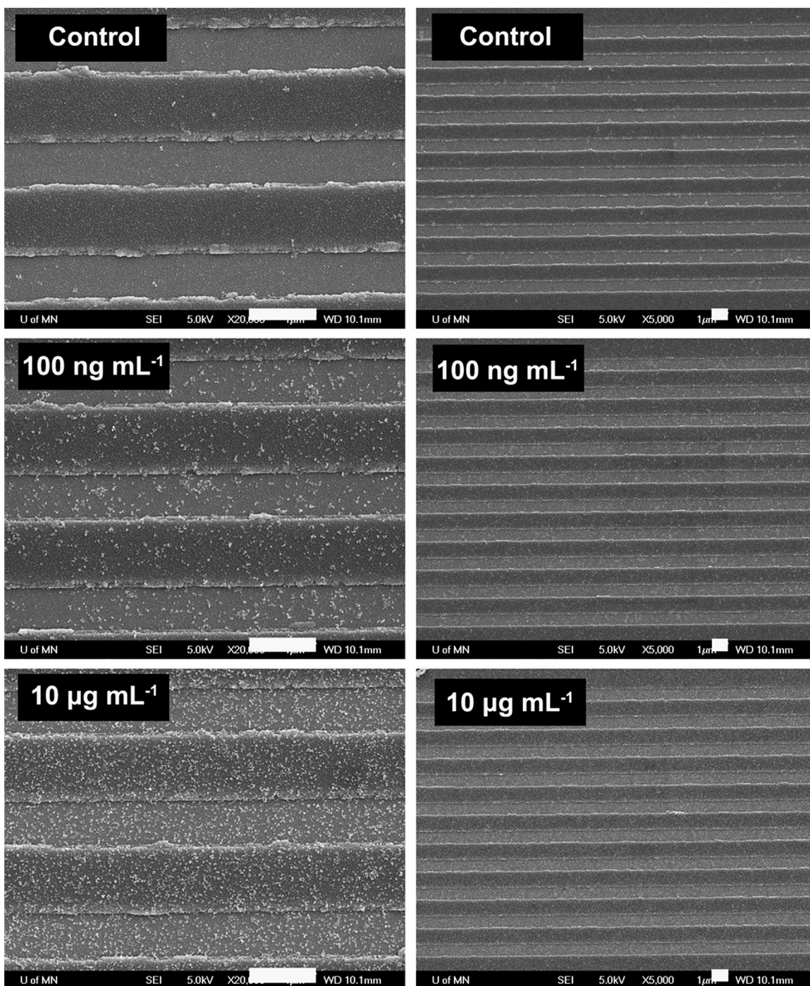
Fig. 3. SEM images of MNPs bound on GMR sensor surface after protein assay. The two upper images show the control sensor surface covered by BSA. Other four images are for PAPP-A assay with different concentrations. All the scale bars are 1 \mu\text{m} .
