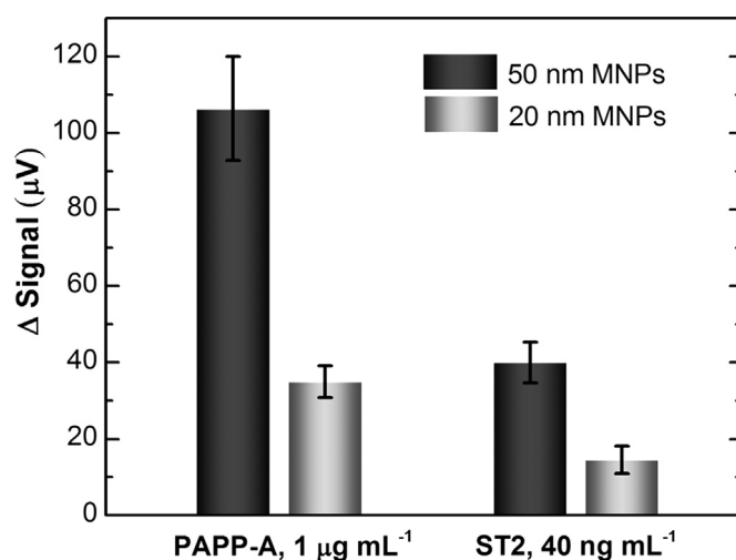
Fig. 4. Comparison of proteins detection using 20 nm MNPs (Ocean NanoTech, SHS-20) and 50 nm MNPs (Miltényi Biotech, MACS 130-048-102).
