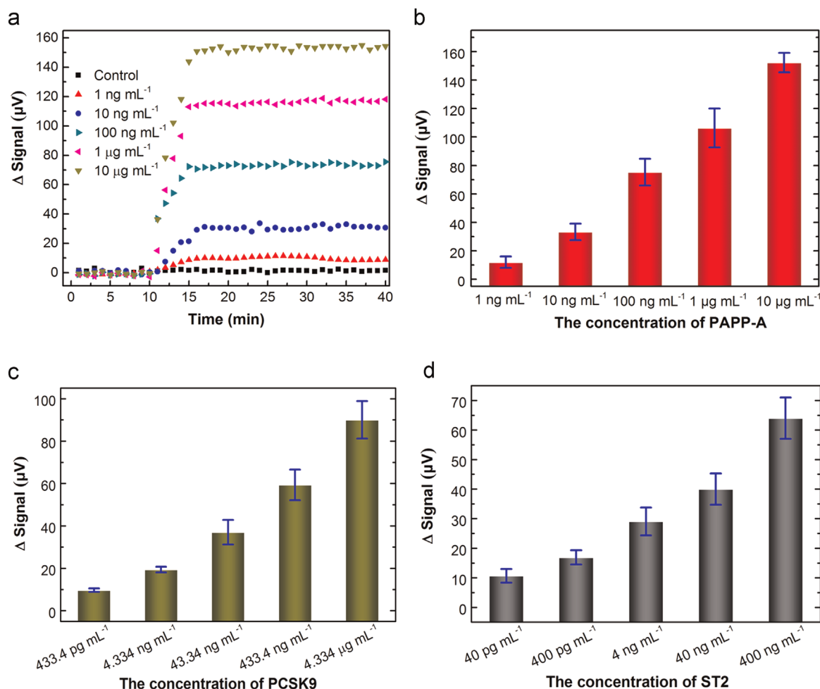
Fig. 2. (a) Typical binding curves in real time and (b) Average final signals (with standard deviation) for PAPP-A antigen. (c) The detection signals (with standard deviation) for PCSK9 antigen. (d) The detection signals (with standard deviation) for ST2 antigen.
