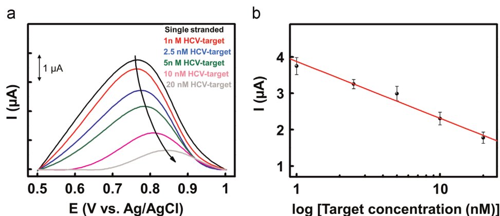
Fig. 5. Sensor response to a range of concentrations of HCV-target. a) DPV measurements, conducted between +0.5 V and +1 V (vs. Ag/AgCl reference electrode) at 100 mV/s in 20 mM Tris–HCl buffer at room temperature and b) corresponding calibration curve, where current intensity is plotted against the logarithm of HCV-target concentration. Error bars are the standard deviation of three independent experiments.
