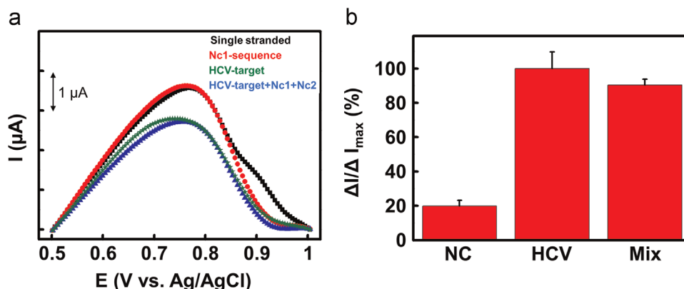
Fig. 4. Selectivity of the DNA sensor. (a) DPV measurements of HCV-modified PEDOT electrodes incubated in hybridization solutions with HCV-target, Nc1-sequence, a mixture of non-complementary sequences (Nc1 + Nc2) and HCV-target, and a DNA-free solution. All DNA sequences were used at a concentration of 50 nM. DPV measurements were conducted between +0.5 V and +1 V (vs. Ag/AgCl reference electrode) at 100 mV/s in 20 mM Tris–HCl buffer at room temperature. (b) Relative current changes of the sensor to different DNA sequences. HCV shows the response of the sensor to the complementary sequence (taken as reference, 100%). Nc1 shows the response of the sensor to the non-complementary sequence. Mix shows the response of the sensor to a mixture of non-complementary (Nc1, Nc2) and complementary sequences. Error bars are the standard deviation of three independent measurements.
