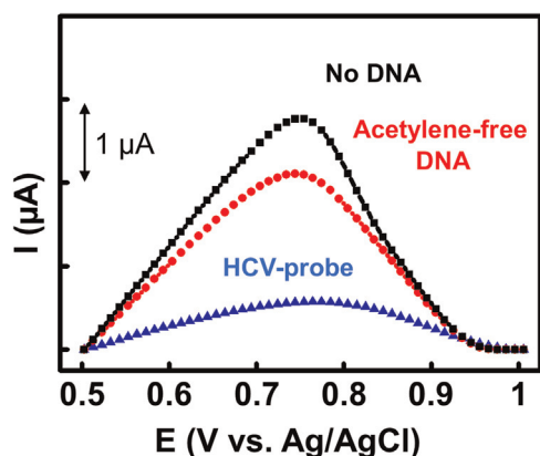
Fig. 3. DPV after “click” reaction. “Click”-functionalized electrodes (blue triangles) showed a decreased current intensity in comparison with azido-PEDOT electrodes that had been incubated with acetylene-free DNA (red dots), and a DNA-free solution (black squares). DPV measurements were conducted between +0.5 V and +1 V (vs. Ag/AgCl reference electrode) at 100 mV/s in 20 mM Tris–HCl buffer at room temperature. (For interpretation of the references to color in this figure legend, the reader is referred to the web version of this article.)
